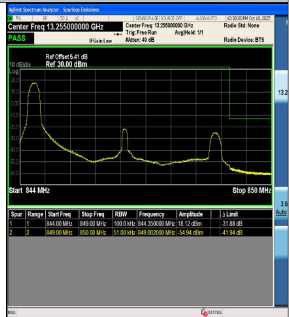
Band26(824-849)-5MHz-16QAM-27015-25RB#0-P
