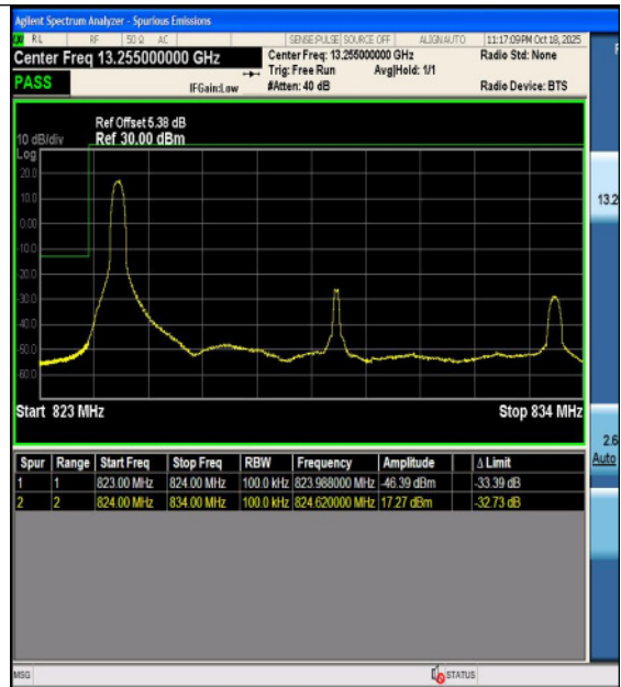
Band26(824-849)-10MHz-16QAM-26840-50RB#0-PASS
