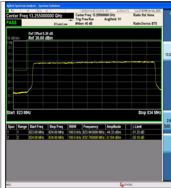
Band26(824-849)-10MHz-16QAM-26840-1RB#49-PASS
