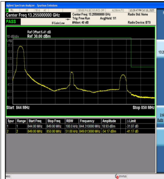
Band26(824-849)-5MHz-QPSK-27015-25RB#0-P
