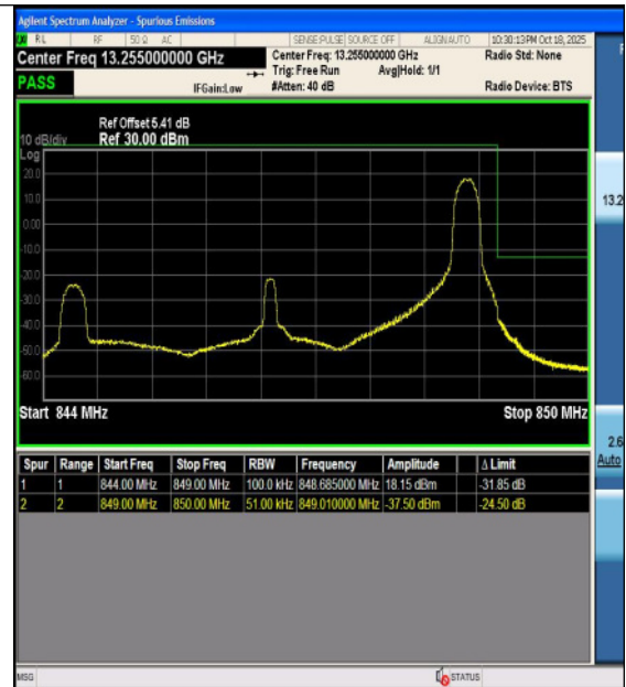
Band26(824-849)-5MHz-16QAM-27015-1RB#0-P
