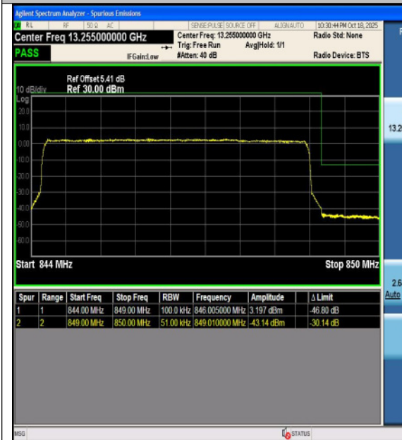
Band26(824-849)-5MHz-16QAM-27015-1RB#24-P
