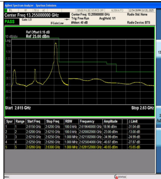
Band38-5MHz-16QAM-38225-1RB#0-PASS
