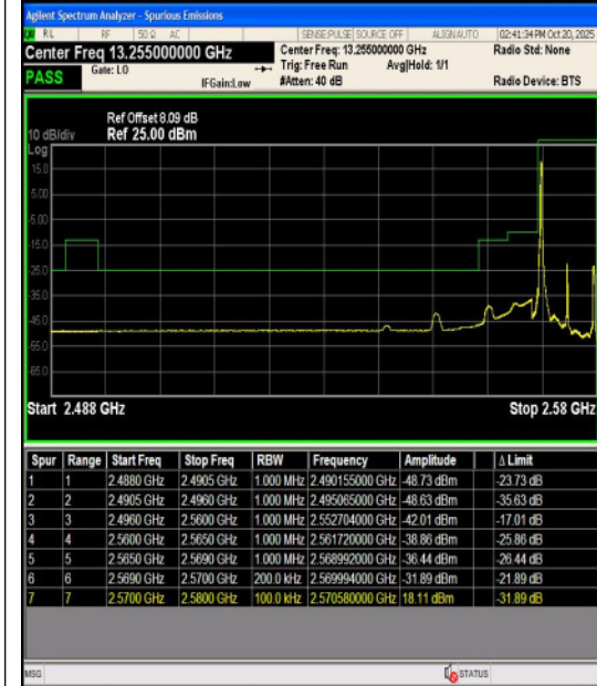
Band38-10MHz-QPSK-37800-50RB#0-PASS
