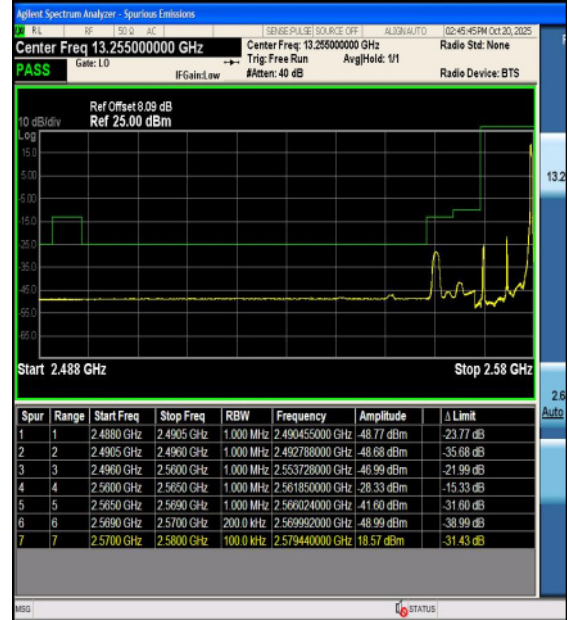
Band38-10MHz-16QAM-37800-1RB#0-PASS
