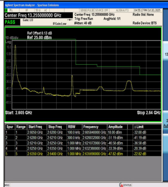
Band38-15MHz-16QAM-38175-75RB#0-PASS
