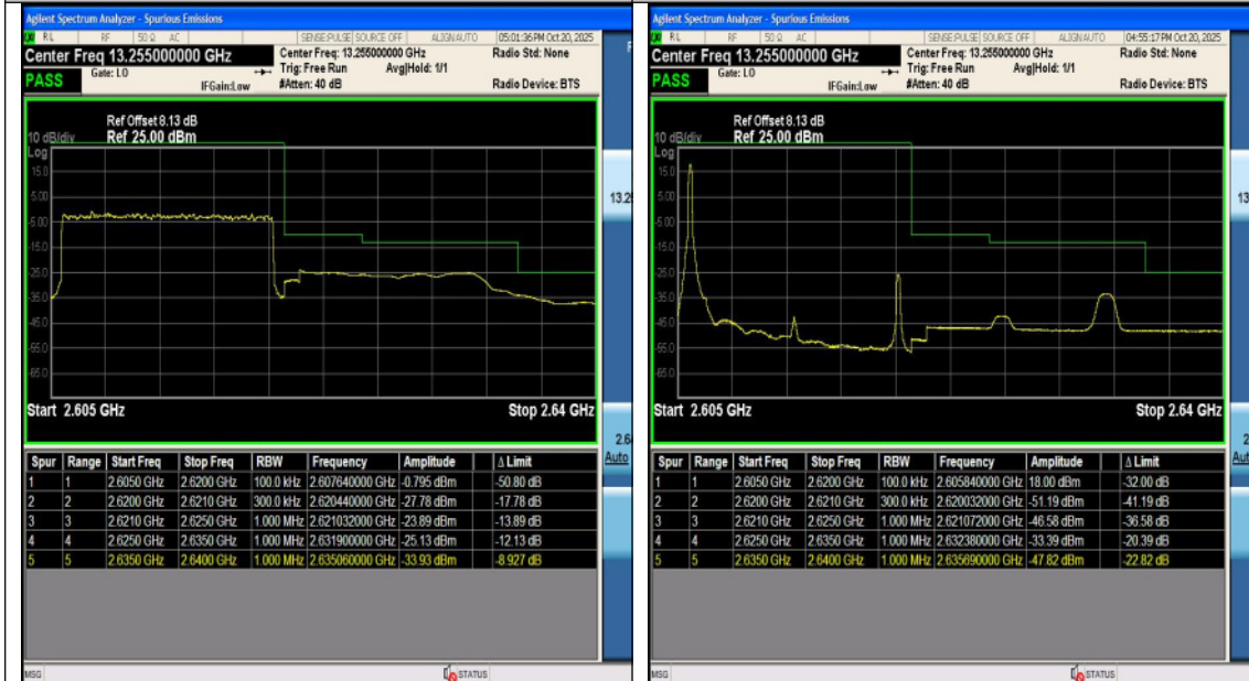
Band38-15MHz-16QAM-38175-1RB#74-PASS
