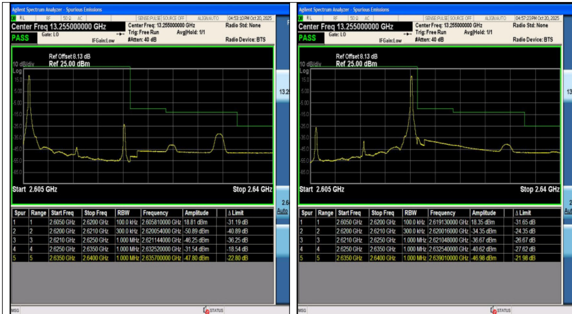
Band38-15MHz-QPSK-38175-75RB#0-PASS
