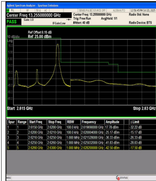
Band38-10MHz-QPSK-37800-1RB#0-PASS
