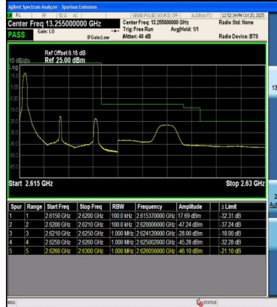
Band38-5MHz-16QAM-38225-25RB#0-PASS
