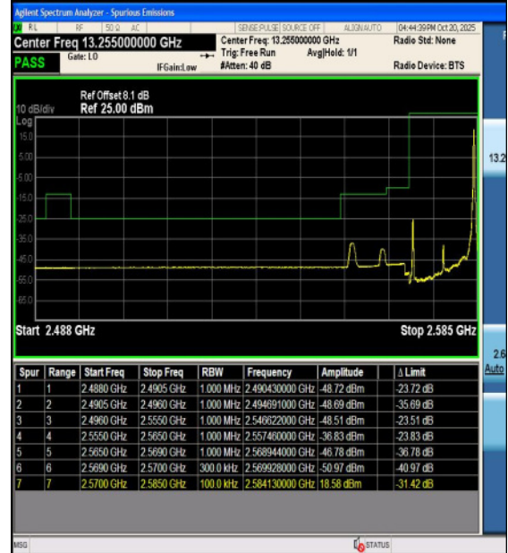
Band38-15MHz-16QAM-37825-1RB#0-PASS
