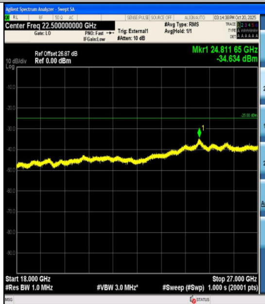
Band38-10MHz-16QAM-37800-1RB#49-0.15~30 -PASS
