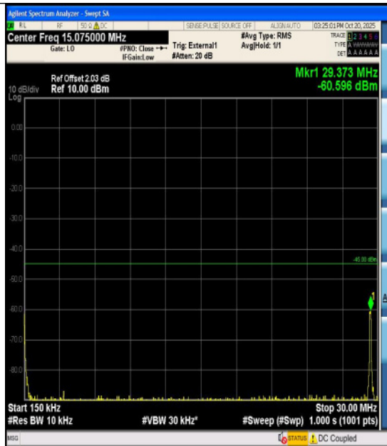
Band38-10MHz-QPSK-38000-1RB#0-1000~300 0-PASS
