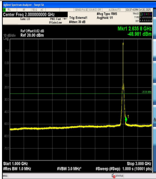
Band38-10MHz-16QAM-38000-50RB#0-18000~ 27000-PASS
