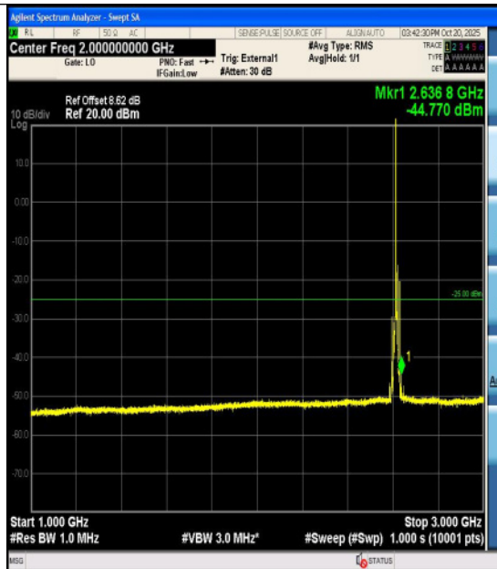
Band38-10MHz-16QAM-38200-1RB#0-18000~2 7000-PASS
