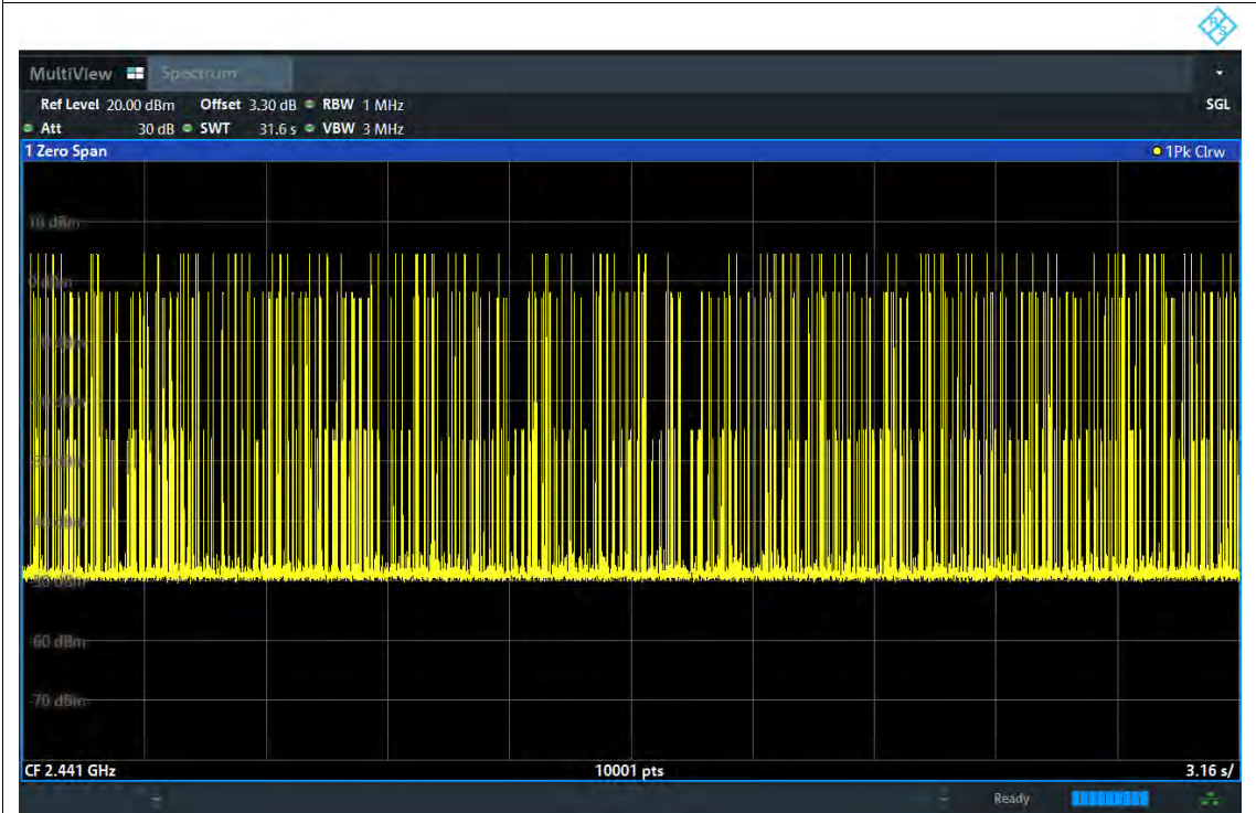
Dwell NVNT 3-DH5 2441MHz Ant1 Accumulated
