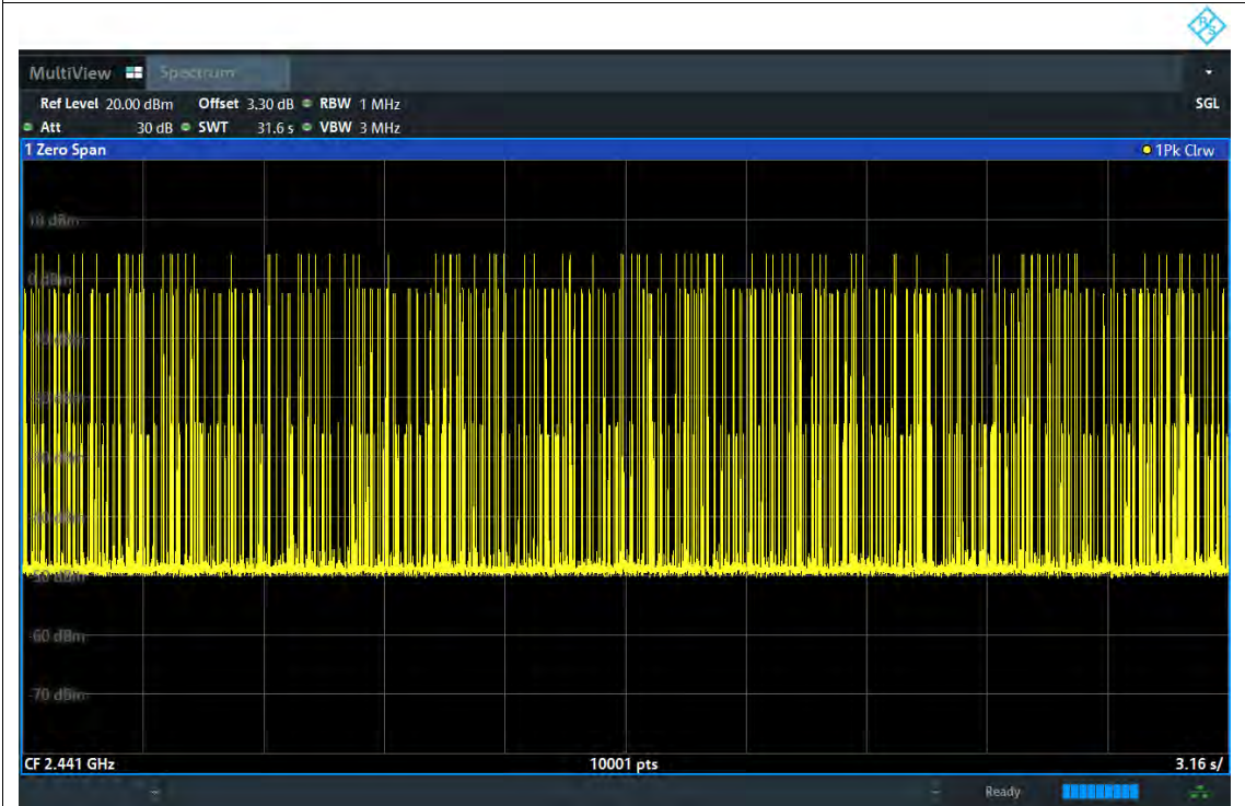
Dwell NVNT 2-DH5 2441MHz Ant1 Accumulated
