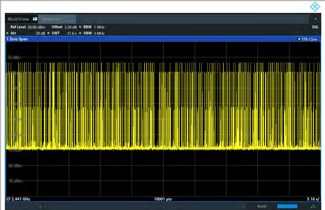
Dwell NVNT 2-DH3 2441MHz Ant1 Accumulated
