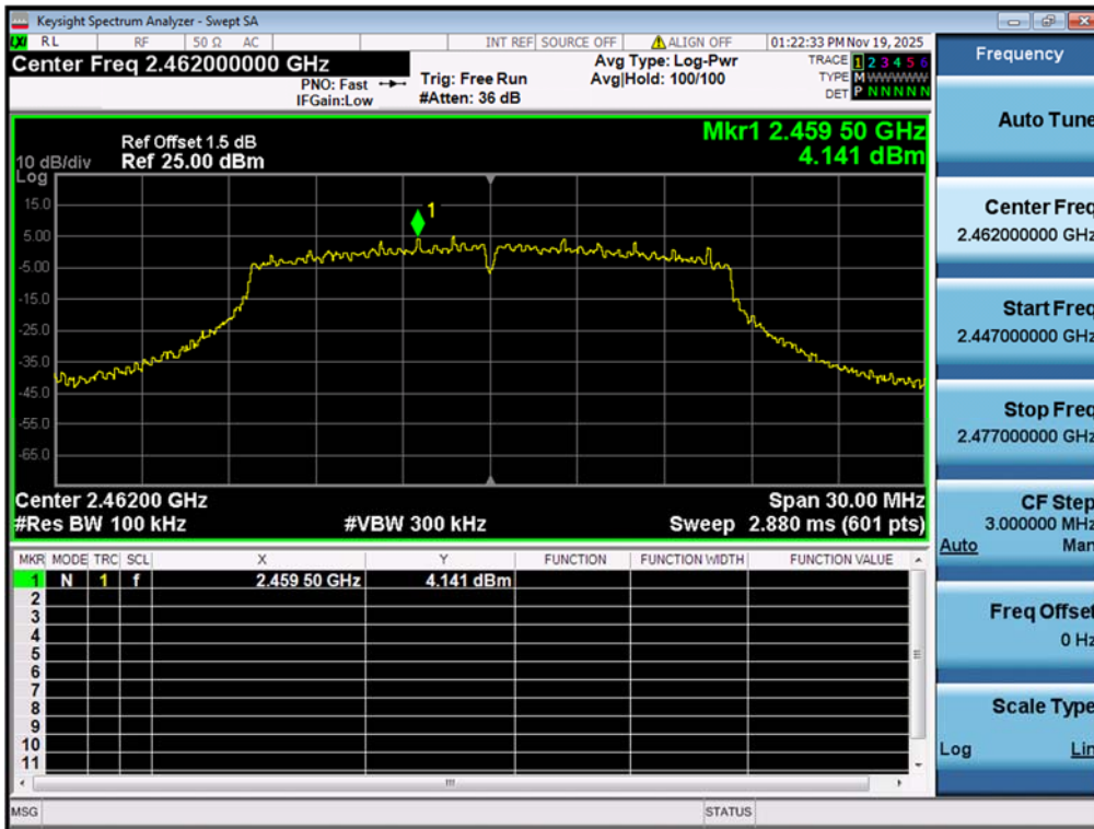
Figure 34: Conducted Spurious Emission & Authorized-band band-edge, 802.11g, 2462MHz Carrier Level
