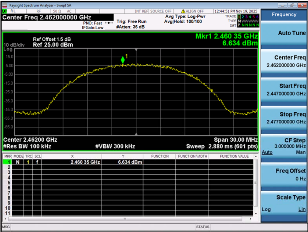
Figure 31: Conducted Spurious Emission & Authorized-band band-edge, 802.11b, 2462MHz Carrier Level
