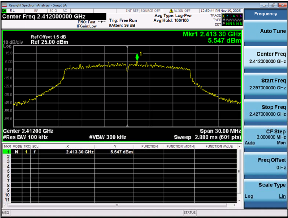
Figure 32: Conducted Spurious Emission & Authorized-band band-edge, 802.11g, 2412MHz Carrier Level
