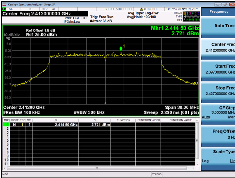
Figure 35: Conducted Spurious Emission & Authorized-band band-edge, 802.11n(HT20), 2412MHz Carrier Level
