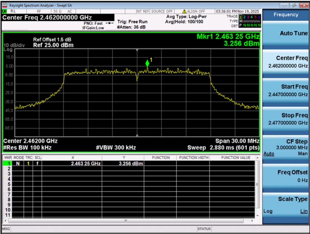
Figure 37: Conducted Spurious Emission & Authorized-band band-edge, 802.11n(HT20), 2462MHz Carrier Level
