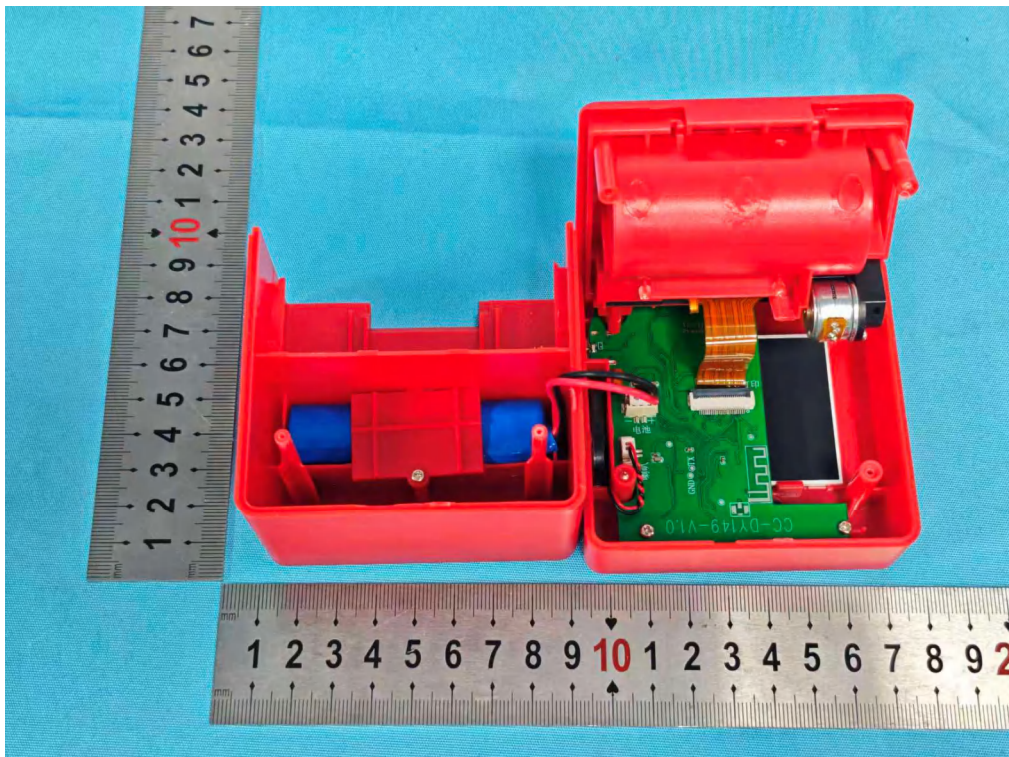
Photo 2 Internal photos of EUT M/N: D5
