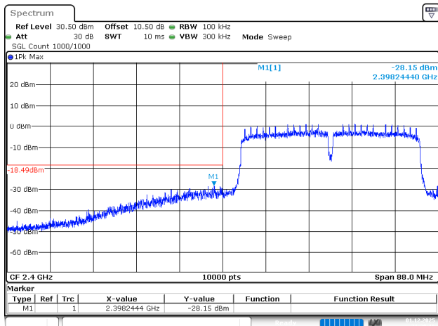
802.11n40_2422MHz
