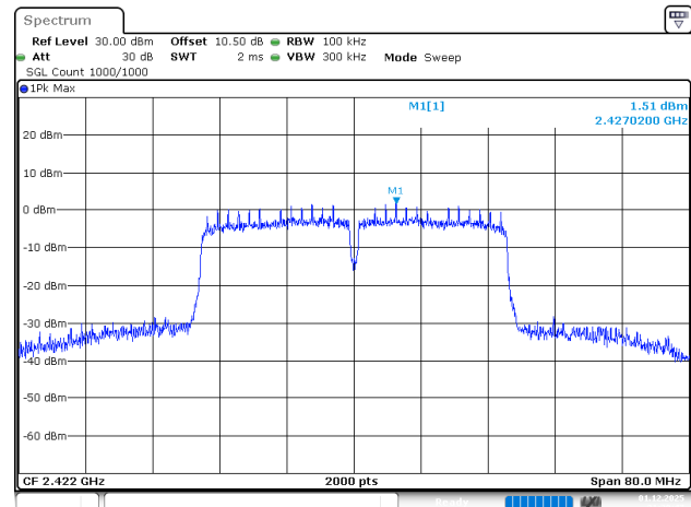
802.11n40_2422MHz
