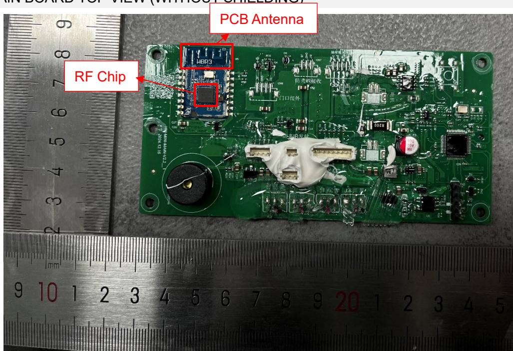
MAIN BOARD TOP VIEW (WITHOUT SHIELDING)
