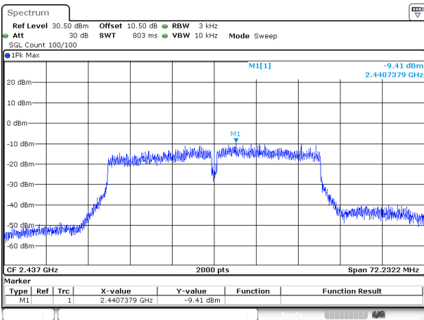
802.11n40_2437MHz
