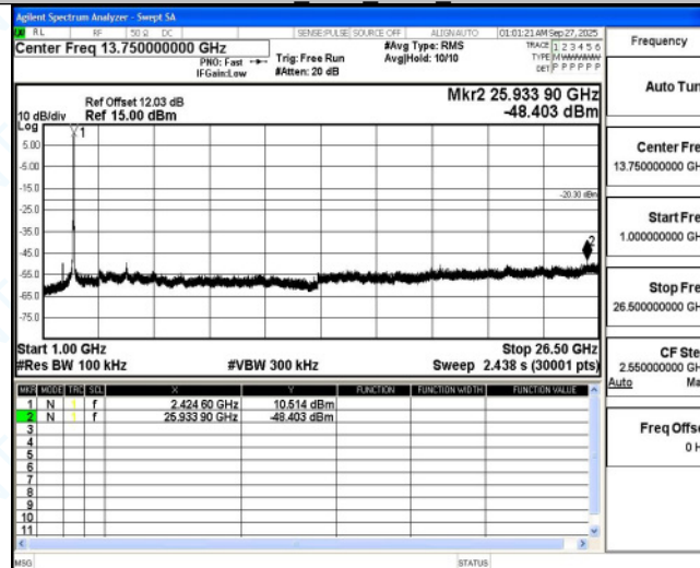
11AX40MIMO Ant2 2422 0~Reference
