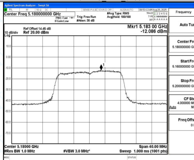
11N20MIMO Ant5 5180
