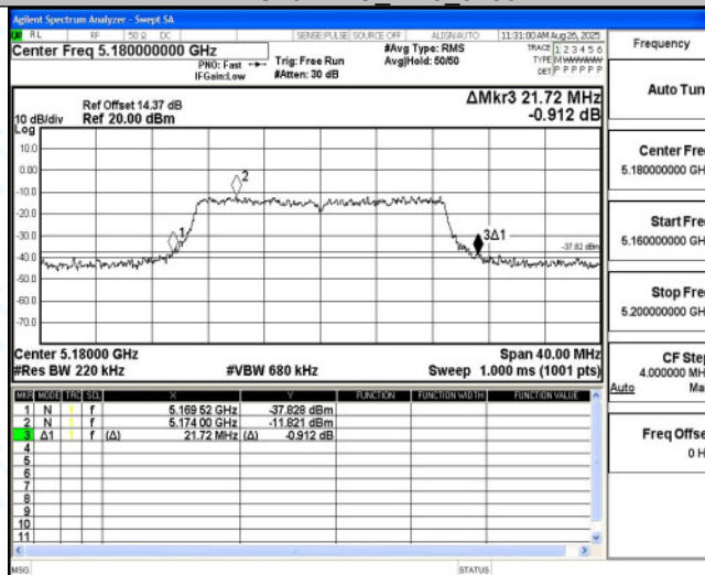
11AC20MIMO_Ant4_5180
