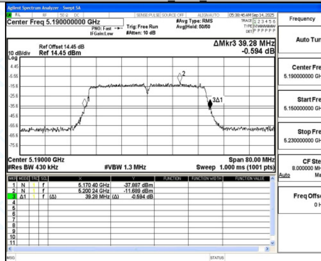
11N40MIMO Ant5 5190
