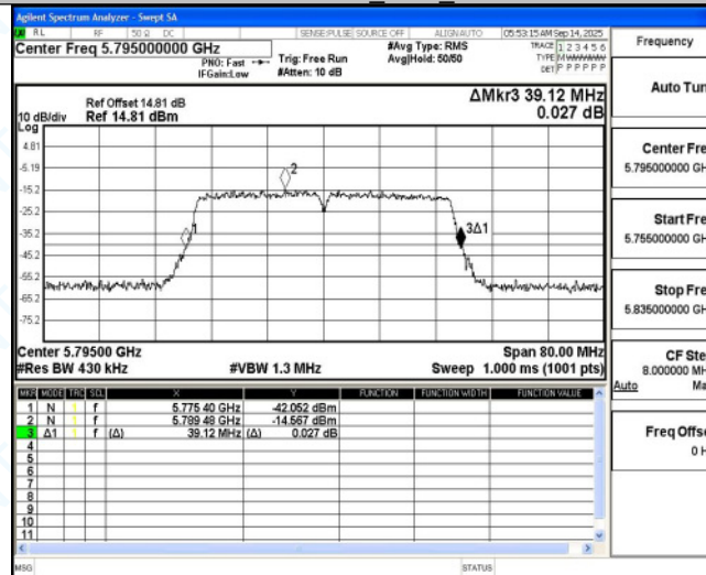
11N40MIMO Ant5 5795
