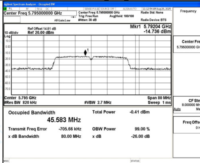
11N40MIMO Ant5 5795
