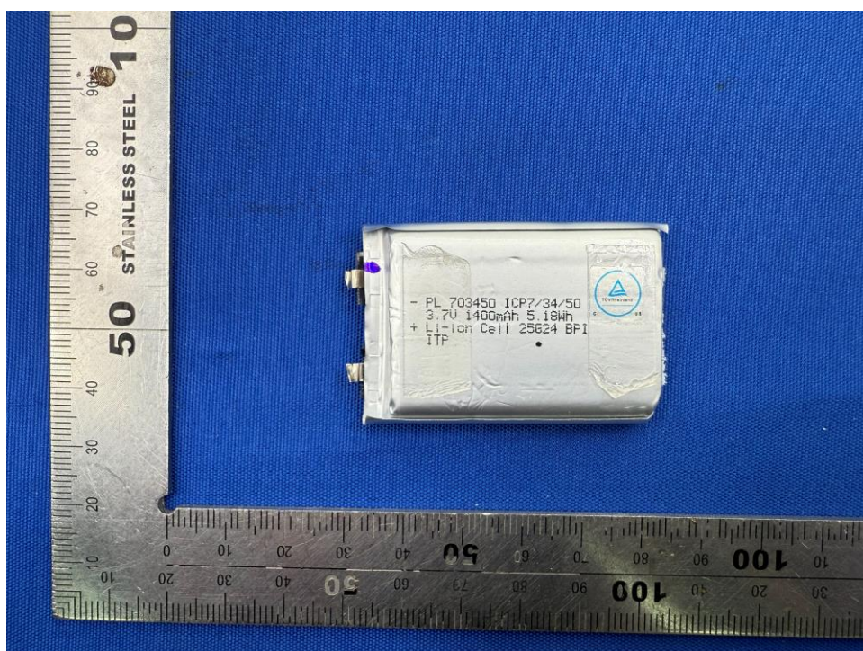
Picture 10. Front view of the component cell_10020
