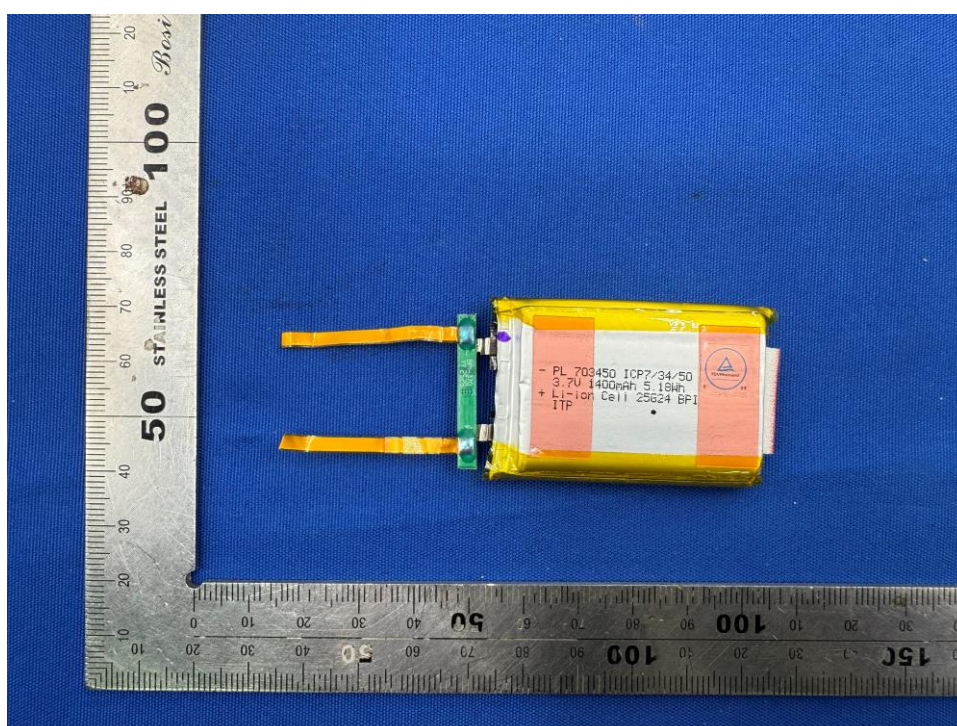
Picture 6. Overview of the PCB D (only for mounting PTC) +cell 10020
