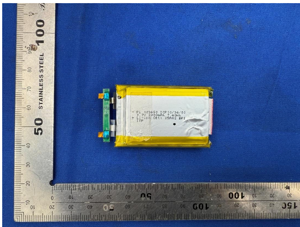
Picture 5. Overview of the PCB D (only for mounting PTC) +cell 10095
