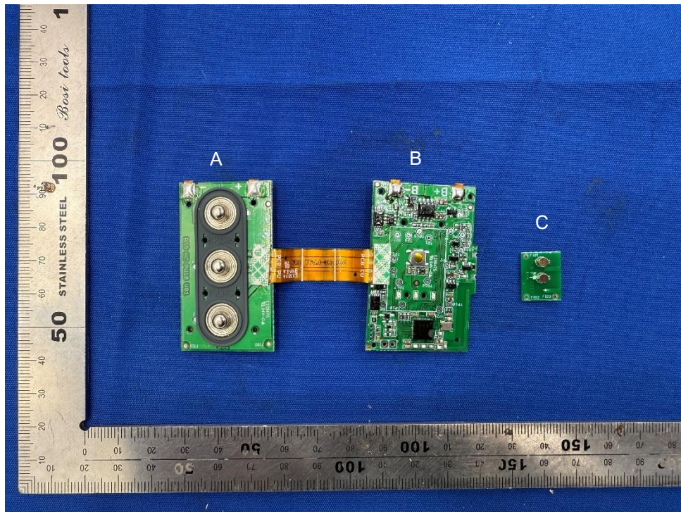
Picture 3. Front view of the PCB A, PCB B, PCB C (10095 & 10020)
