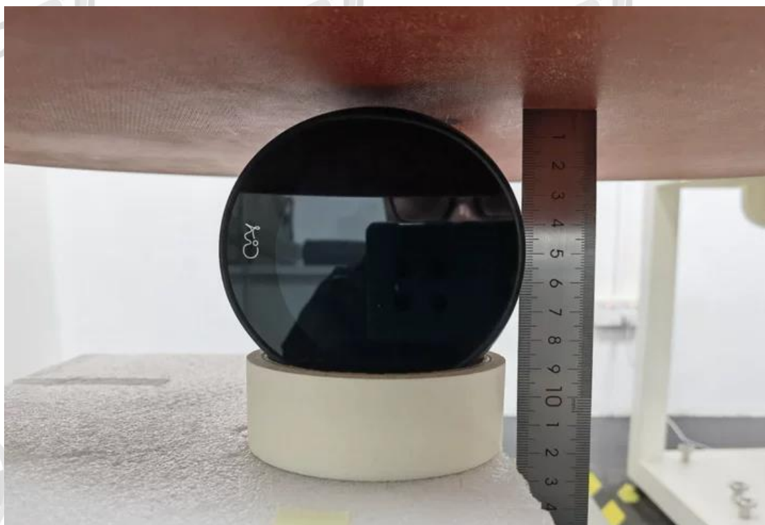
Left Side-5mm
