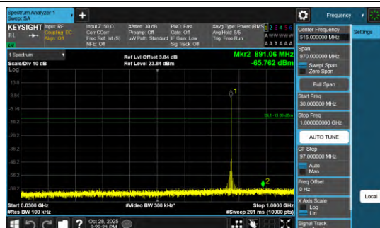
Band13-0.18-QPSK-23181-30-1000-PASS
