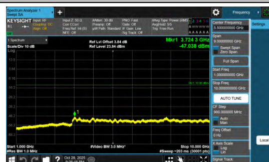
Band13-0.18-QPSK-23181-1000-10000-PASS
