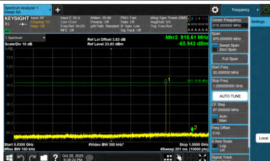
Band13-0.18-QPSK-23279-30-1000-PASS
