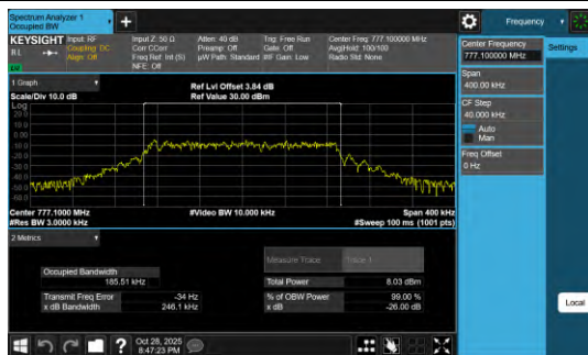
Band13-0.18-QPSK-23181-PASS
