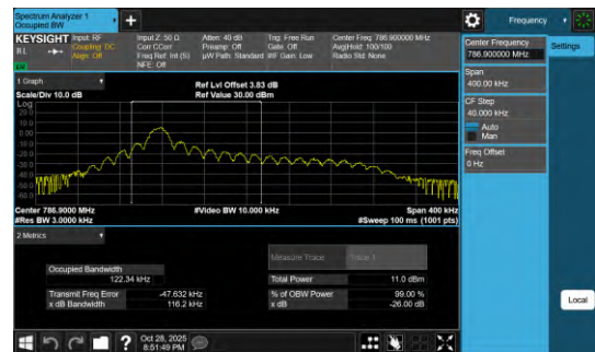
Band13-0.18-QPSK-23279-PASS
