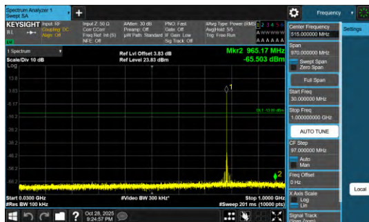
Band13-0.18-QPSK-23279-30-1000-PASS
