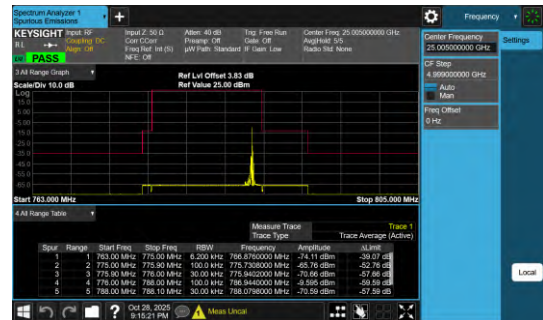
Band13-0.18-QPSK-23279-PASS
