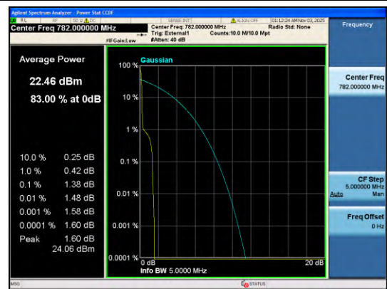
Band13-0.18-QPSK-23230-PASS
