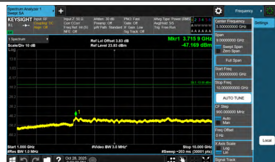
Band13-0.18-BPSK-23279-1000-10000-PASS
