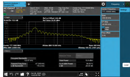
Band13-0.18-QPSK-23181-PASS
