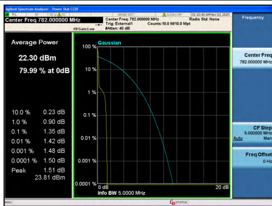
Band13-0.18-QPSK-23230-PASS
