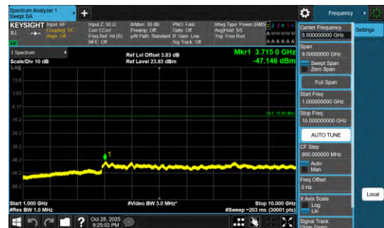
Band13-0.18-QPSK-23279-1000-10000-PASS
