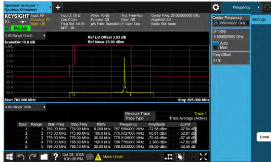
Band13-0.18-QPSK-23279-PASS
