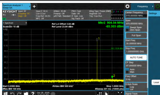
Band13-0.18-BPSK-23181-30-1000-PASS
