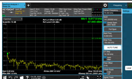
Band13-0.18-QPSK-23230-0.009-0.15-PASS
