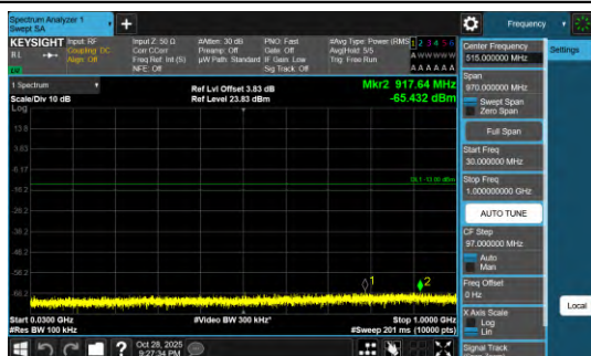
Band13-0.18-QPSK-23230-30-1000-PASS
