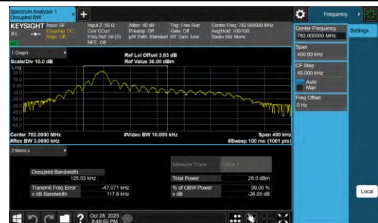
Band13-0.18-QPSK-23230-PASS
