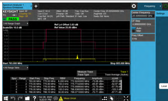
Band13-0.18-QPSK-23279-PASS
