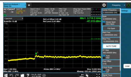
Band13-0.18-QPSK-23230-1000-10000-PASS
