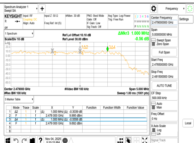
π/4DQPSK_2M_DH5_CH76CH77CH78
