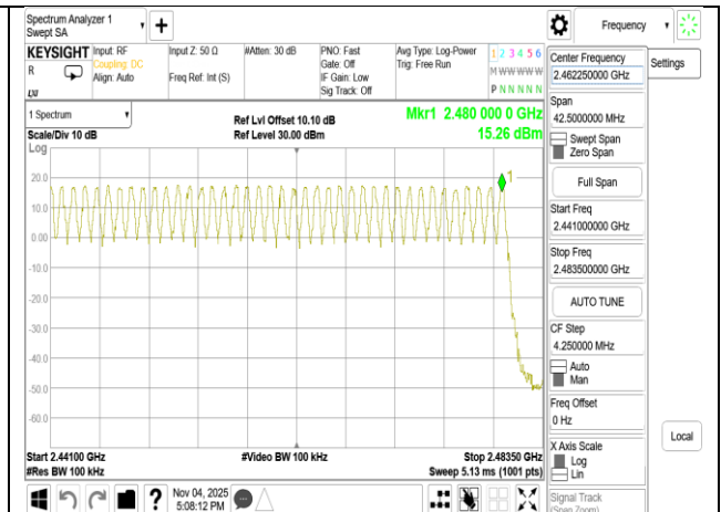
GFSK 1M DH5 2441-2480
