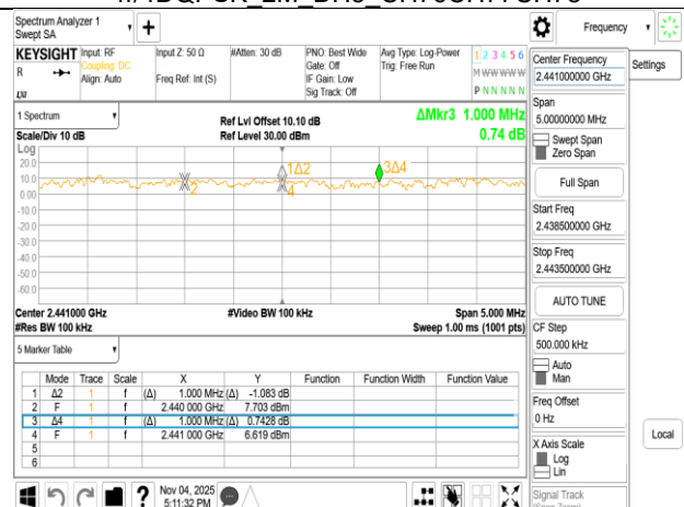
8DPSK_3M_DH5_CH38CH39CH40
