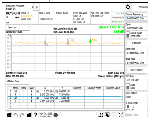
π/4DQPSK_2M_DH5_CH38CH39CH40
