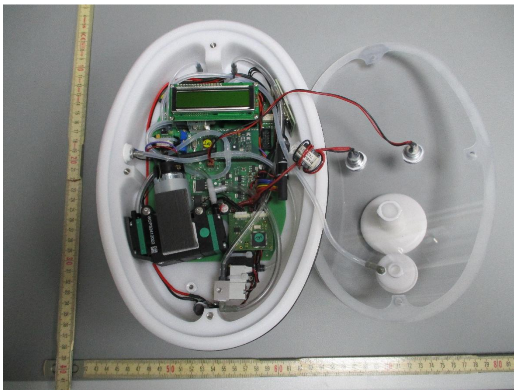
Figure 1: Internal view
