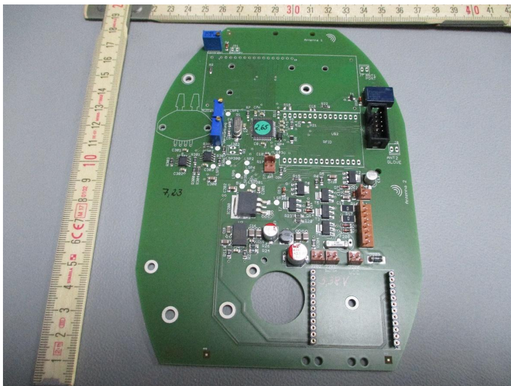
Figure 2: PCB 1
