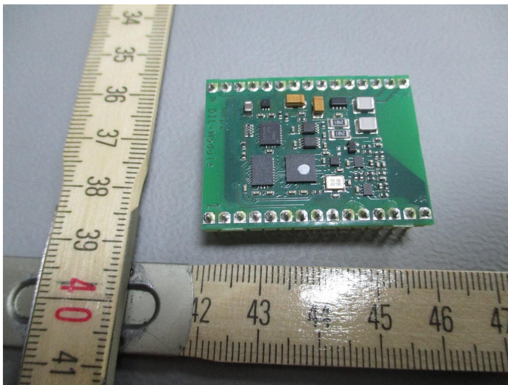
Figure 3: PCB 2
