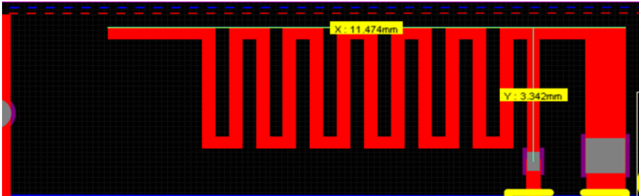
Antenna Dimensions
