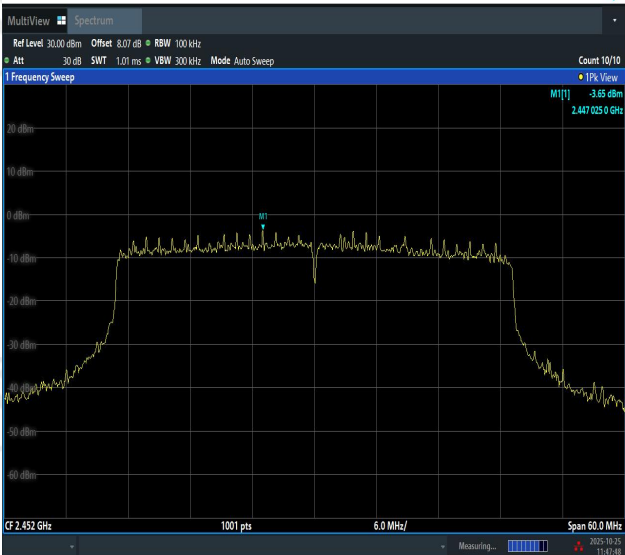
11AX40SISO-Ant1-2452-0~Reference-PASS
