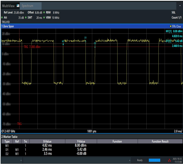
NTNV-11N40SISO-Ant1-2437
