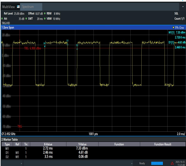
NTNV-11N40SISO-Ant1-2452
