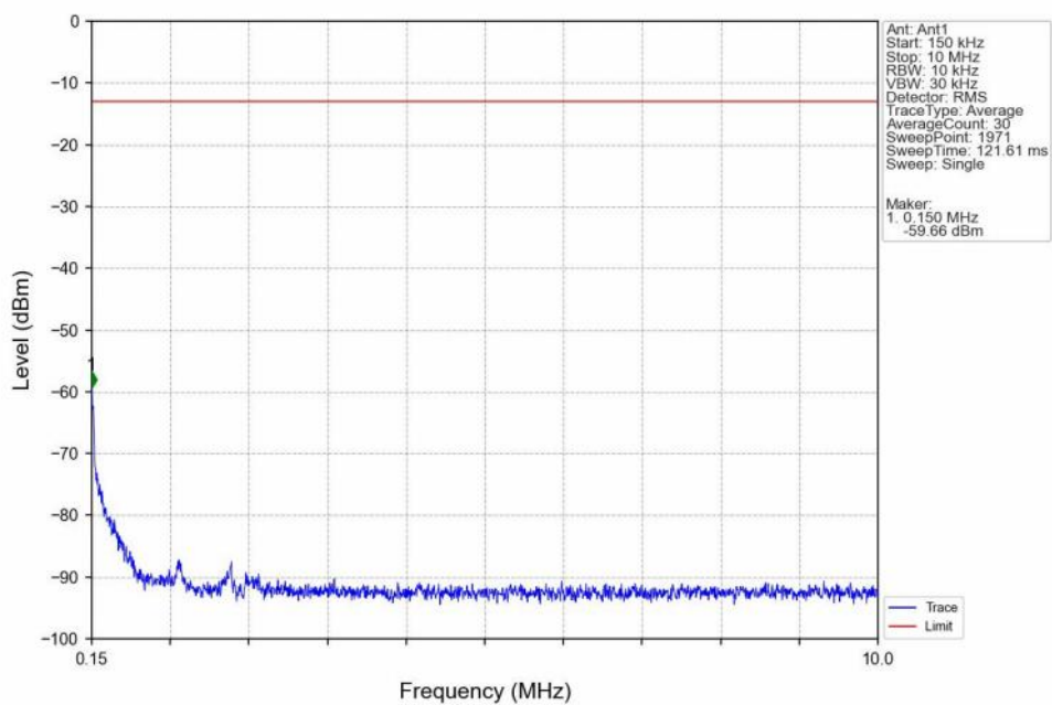
Band12_5MHz_16QAM_HCH_713.5MHz_RB_1_0_NTNV
