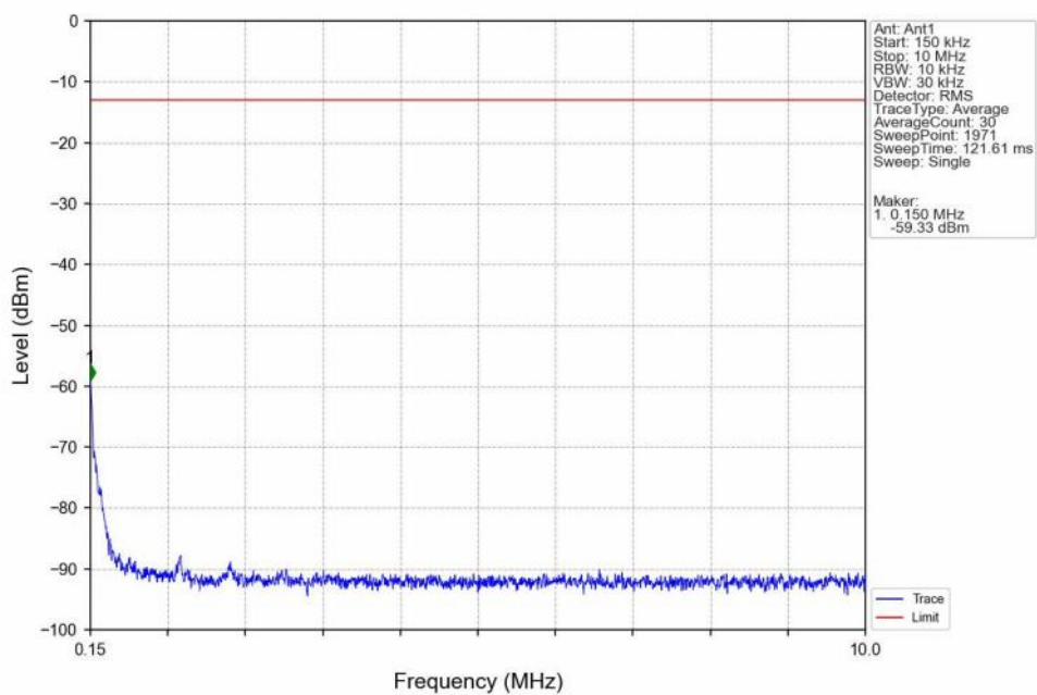
Band12_1.4MHz_16QAM_HCH_715.3MHz_RB_1_0_NTNV
