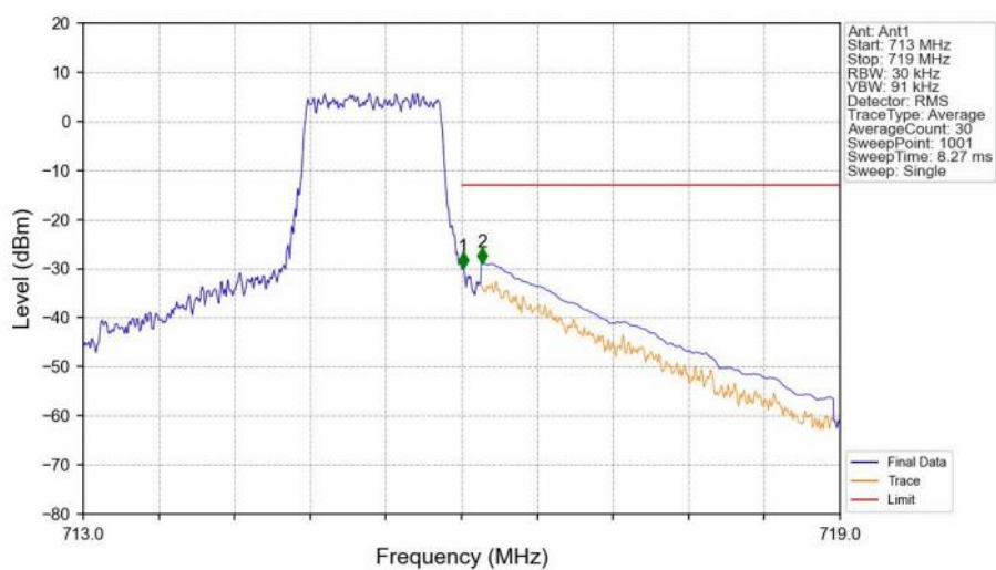
Band12_1.4MHz_16QAM_HCH_715.3MHz_RB_6_0_NTNV
