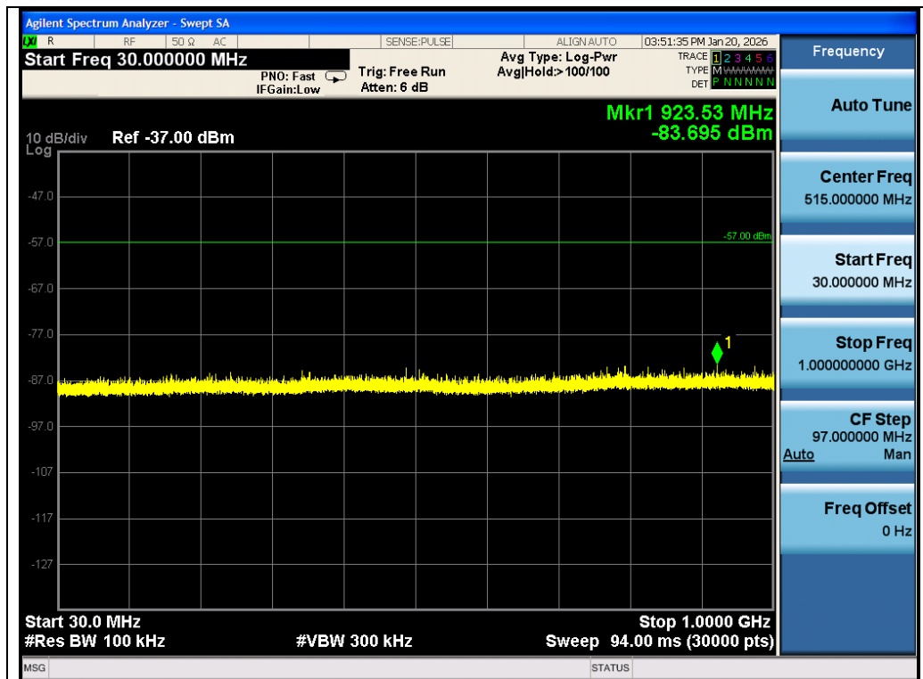
Test_Graph_RX_FrequencyRange_30MHz-1GHz
