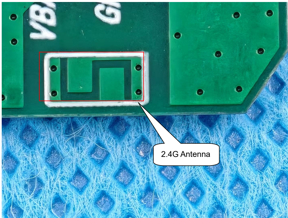
VIEW-2 OF ANTENNA
