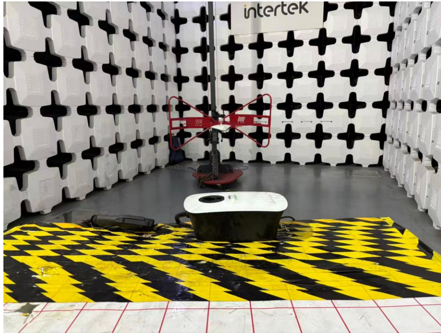
The EUT is placed at the center of turntable (30MHz-1GHz)
