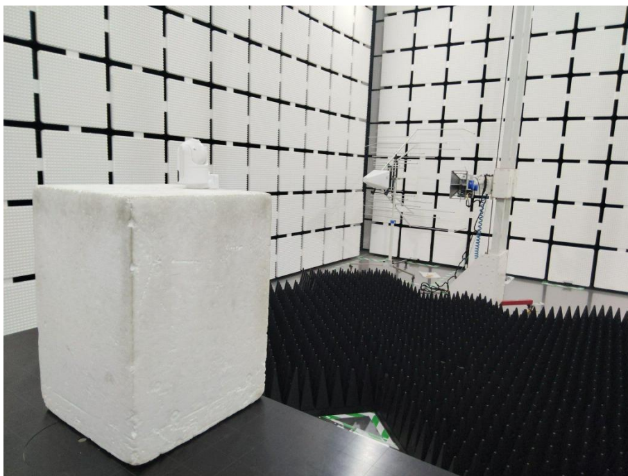
Radiated emissions (UE)(Above 1GHz)
