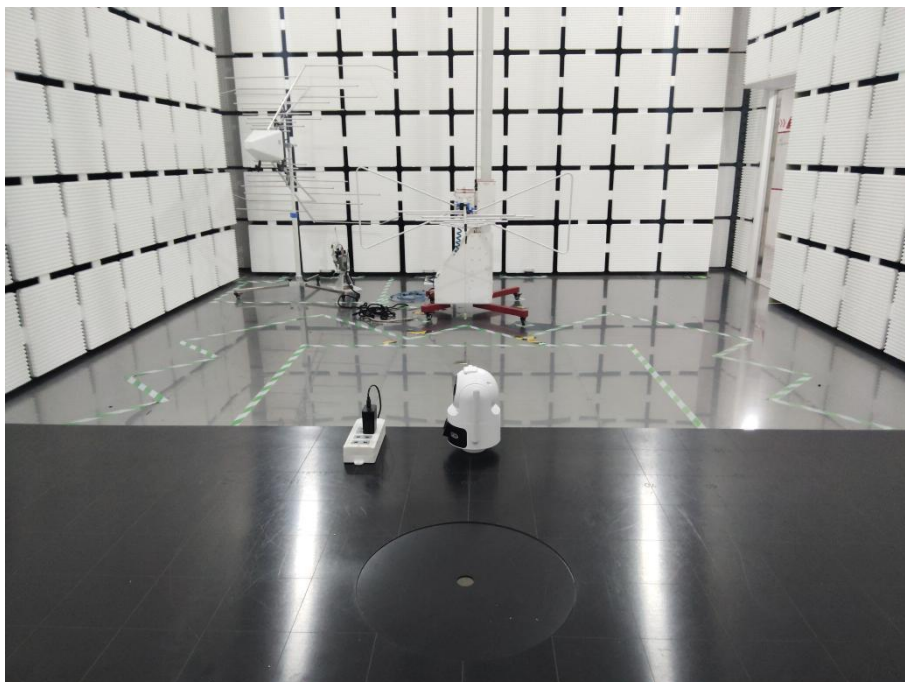
Radiated emissions (UE)(Below 1GHz)
