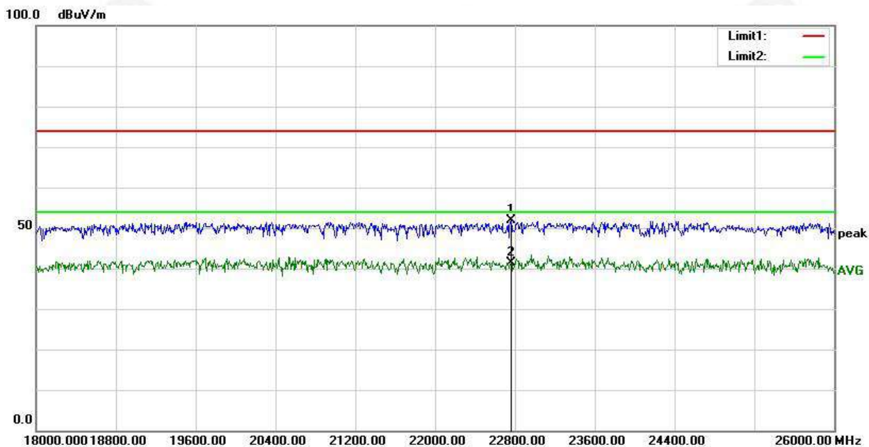
RSE-M-18GHz-26GHz-H
