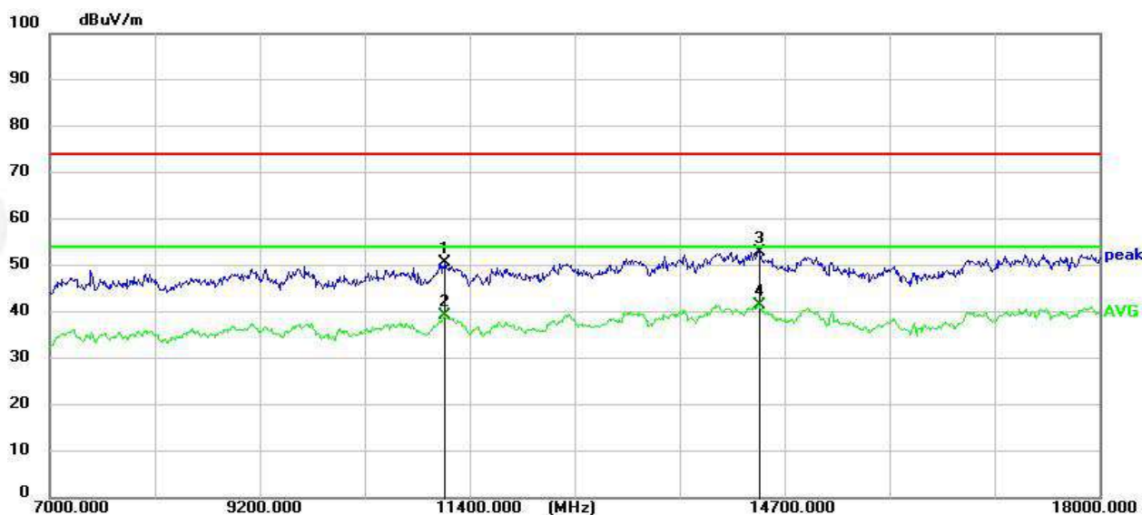
RSE-H-7GHz-18GHz-H
