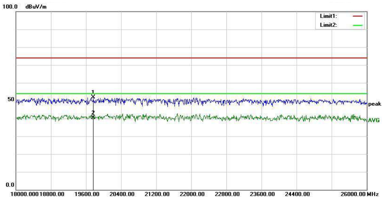
RSE-H-18GHz-26GHz-H
