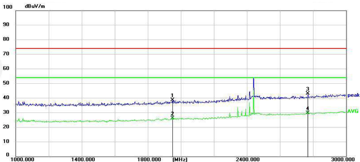
RSE-M-1GHz-3GHz-H
