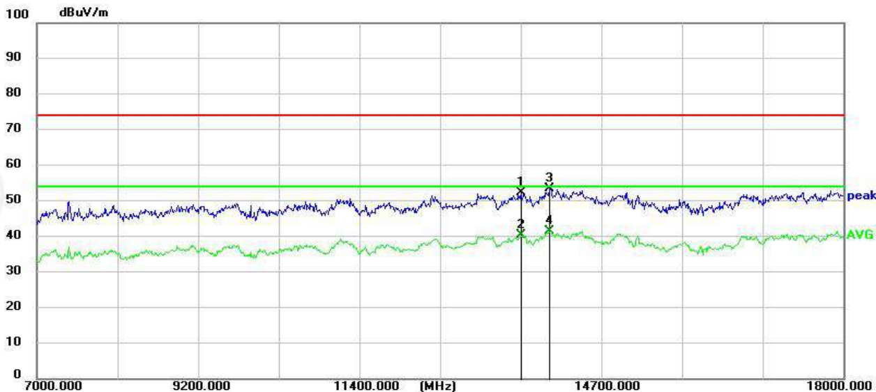
RSE-H-7GHz-18GHz-H
