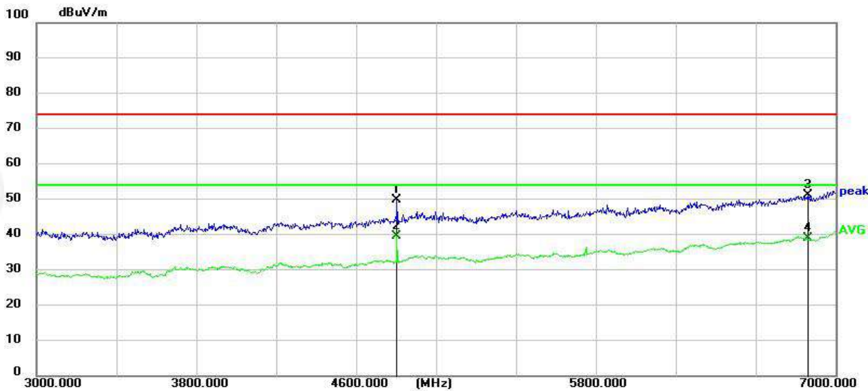
RSE-L-3GHz-7GHz-H
