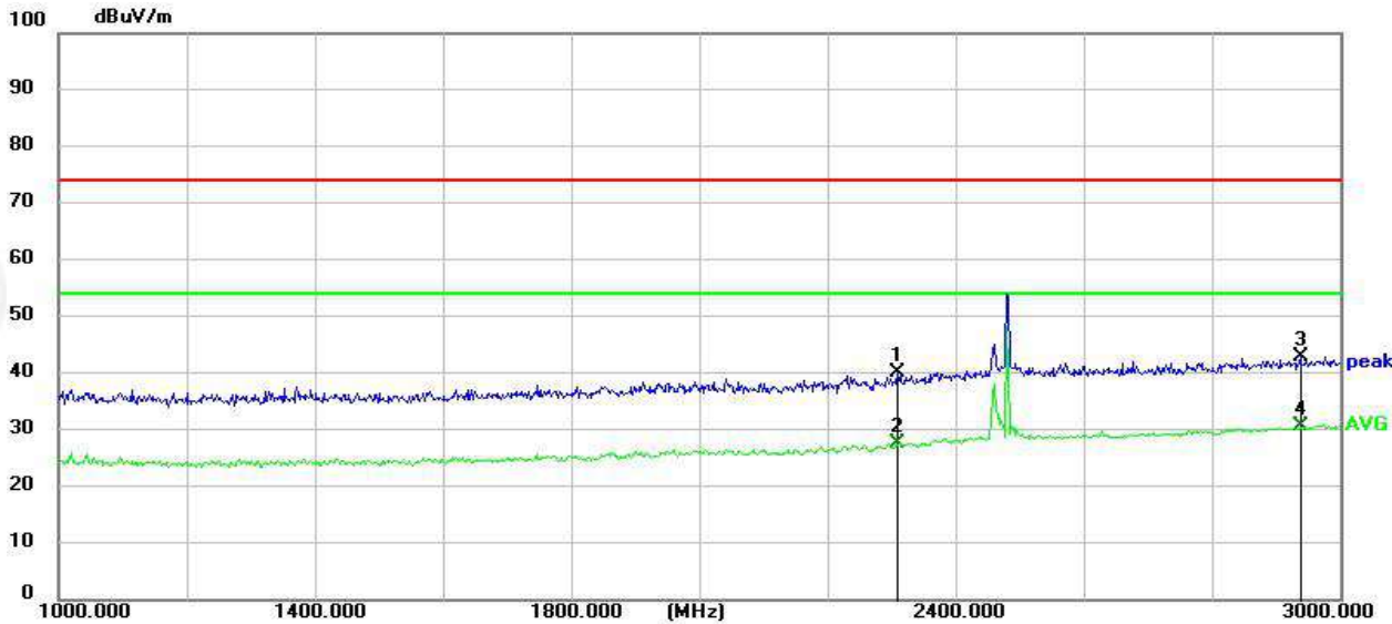
RSE-H-1GHz-3GHz-H
