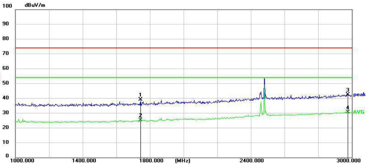
RSE-H-1GHz-3GHz-H
