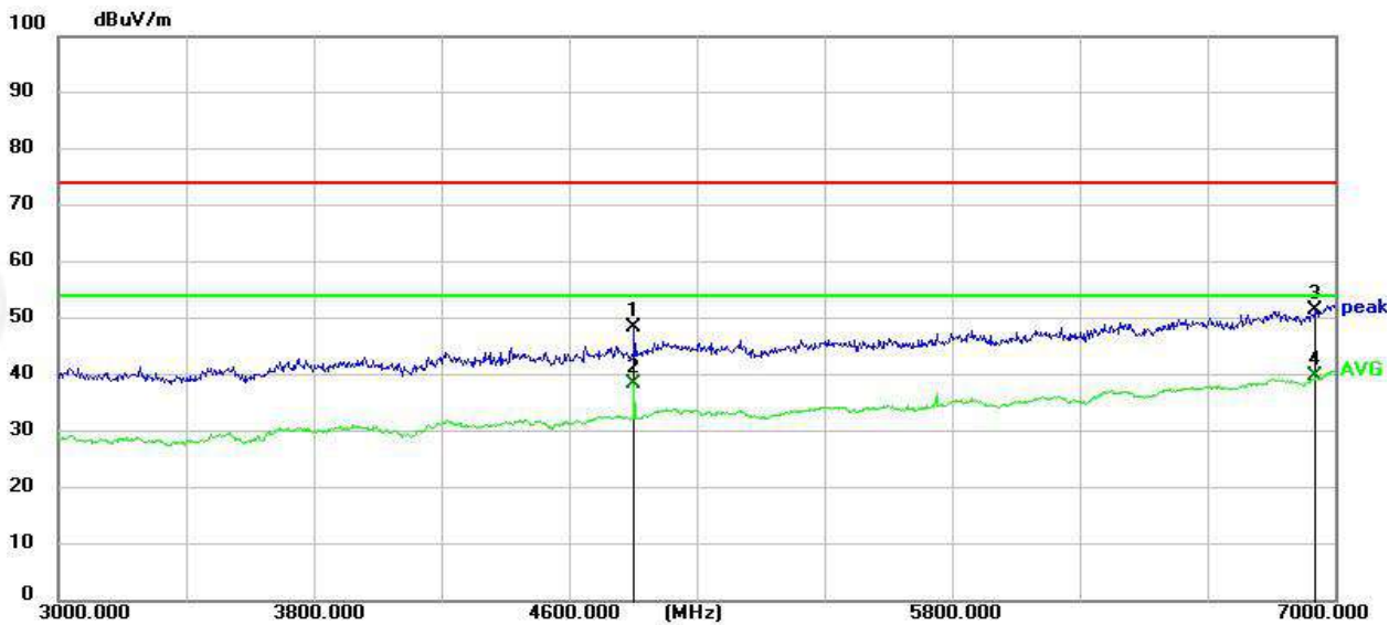
RSE-L-3GHz-7GHz-H
