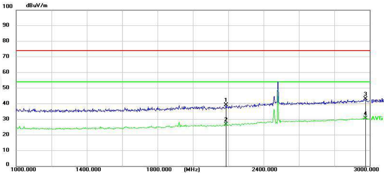
RSE-H-1GHz-3GHz-H
