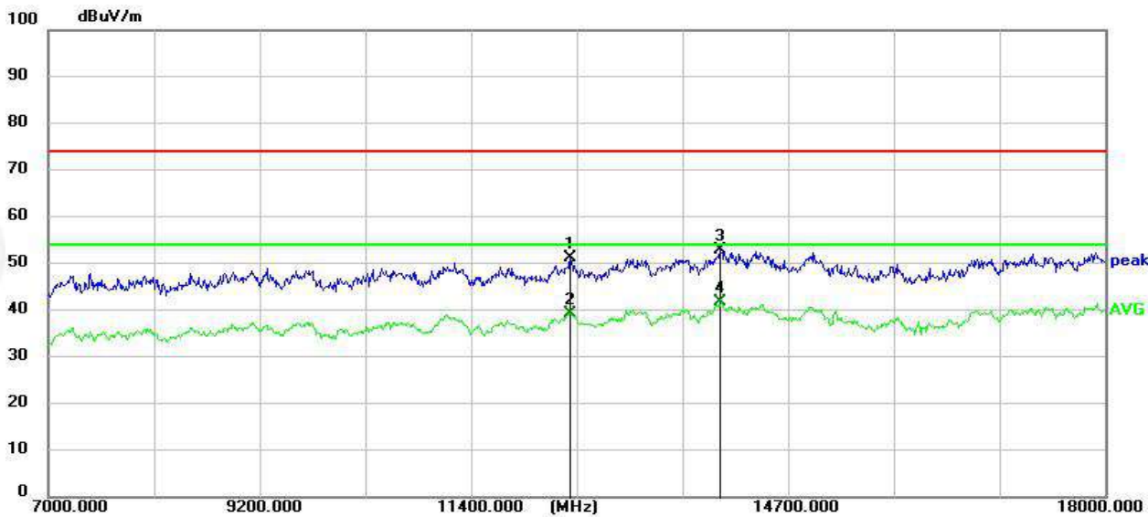
RSE-H-7GHz-18GHz-H
