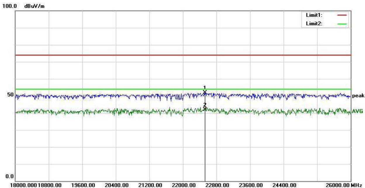
RSE-M-18GHz-26GHz-H
