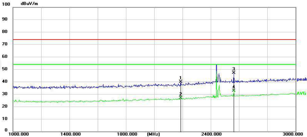
RSE-M-1GHz-3GHz-H
