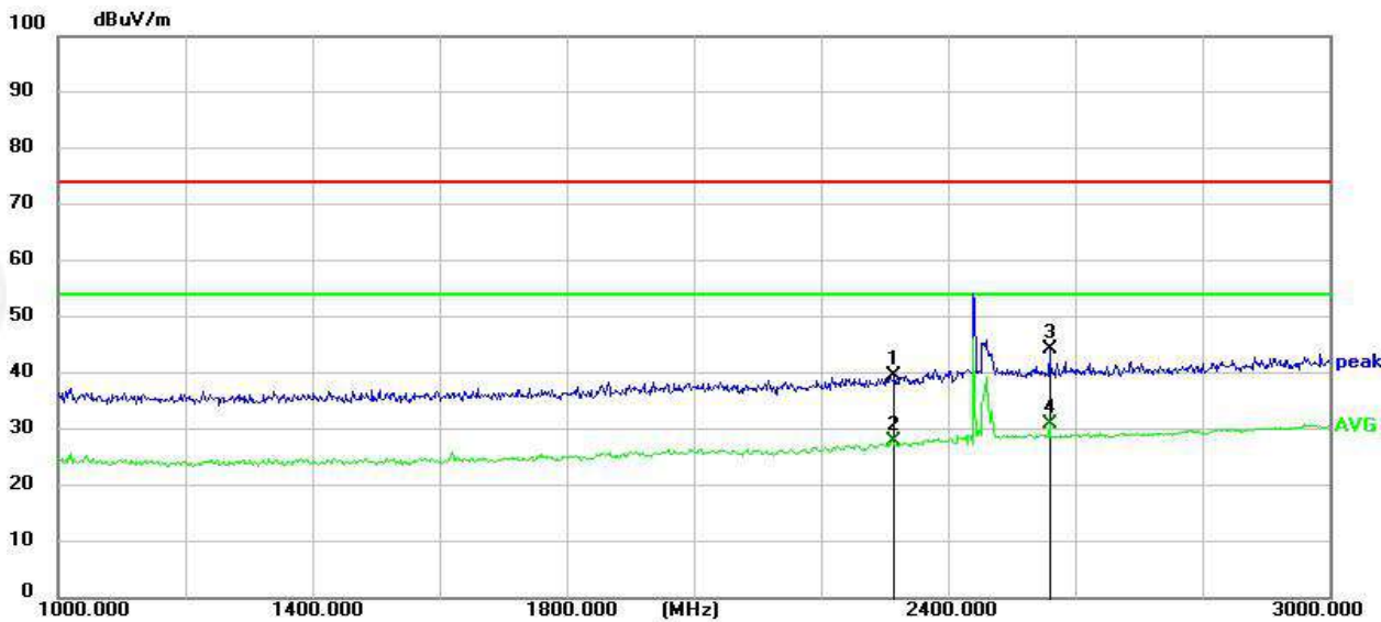
RSE-M-1GHz-3GHz-H
