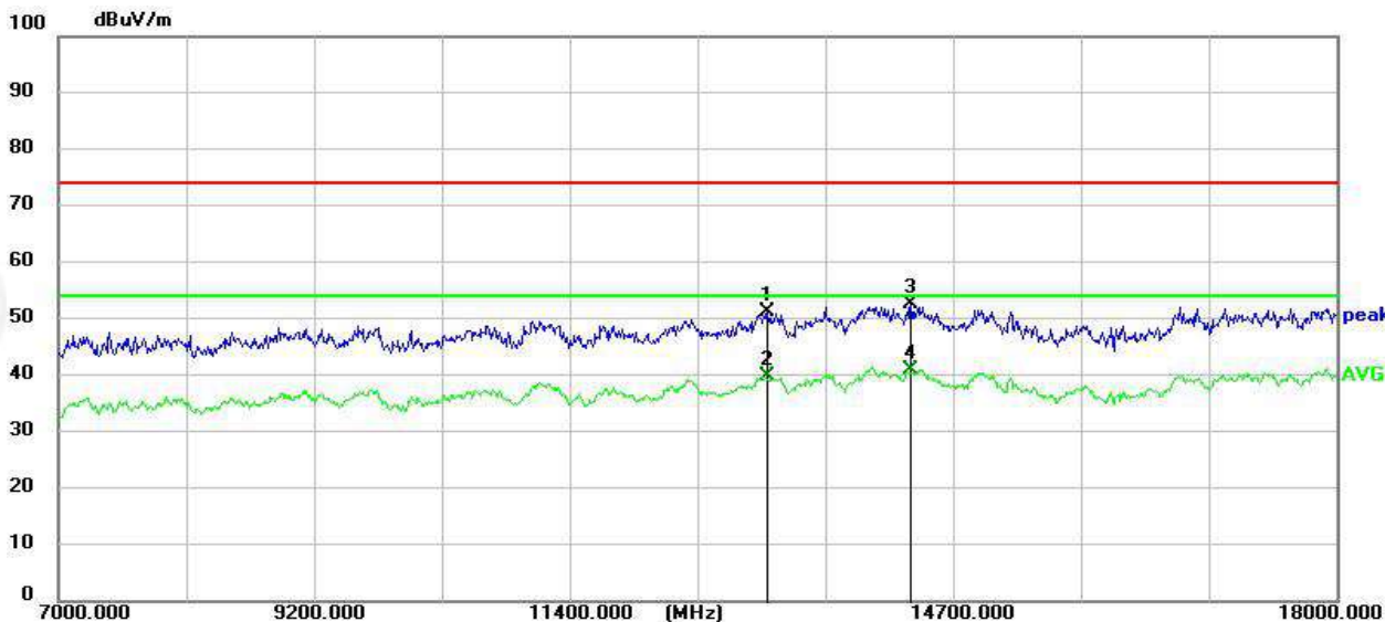
RSE-H-7GHz-18GHz-H
