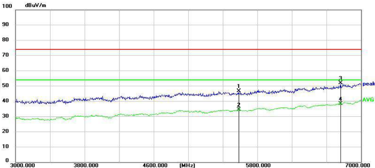
RSE-L-3GHz-7GHz-H
