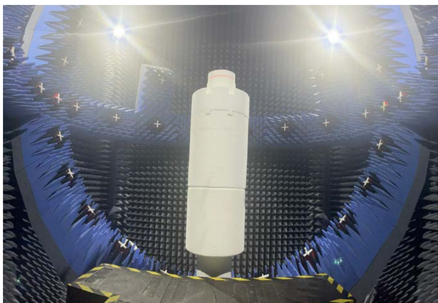
Figure 1 – RayZone-5000M. The DUT is placed on top of the pedestal, in the center of the system.
