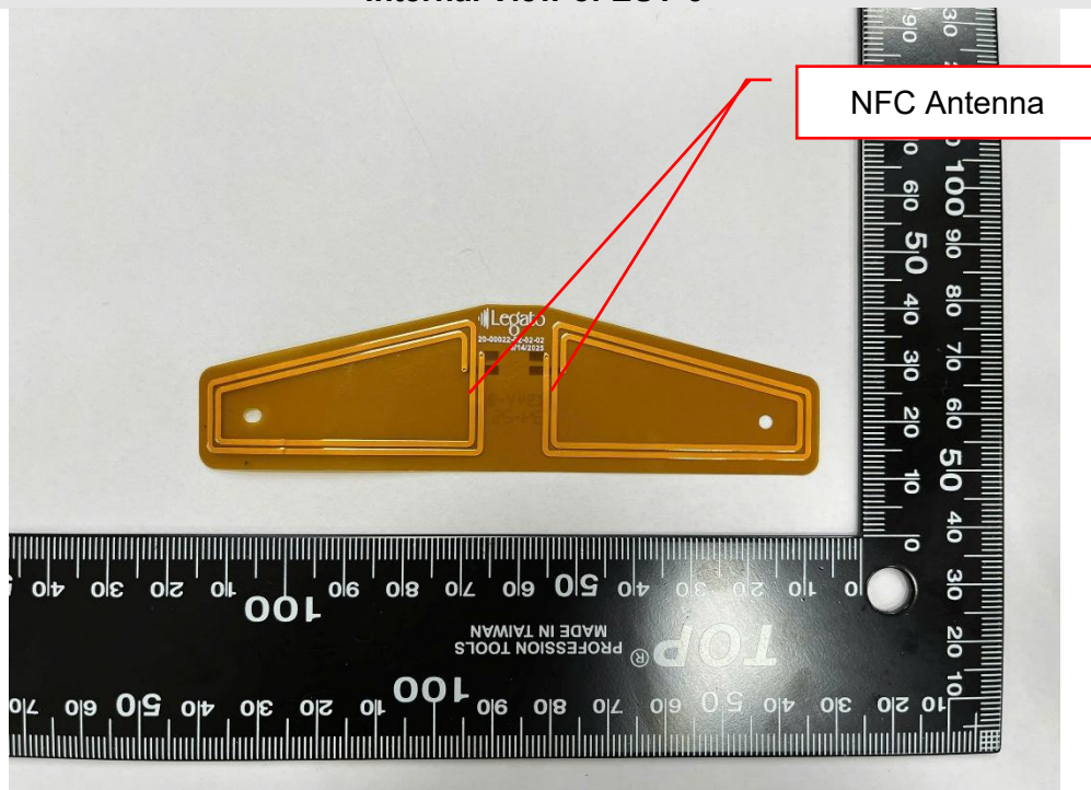
Internal View of EUT-6
