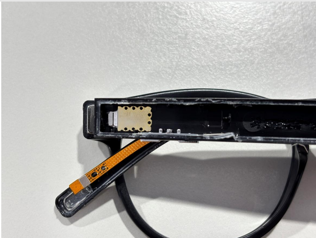
Left Frame Internal View of EUT-17
