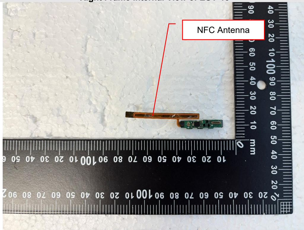
Right Frame Internal View of EUT-14
