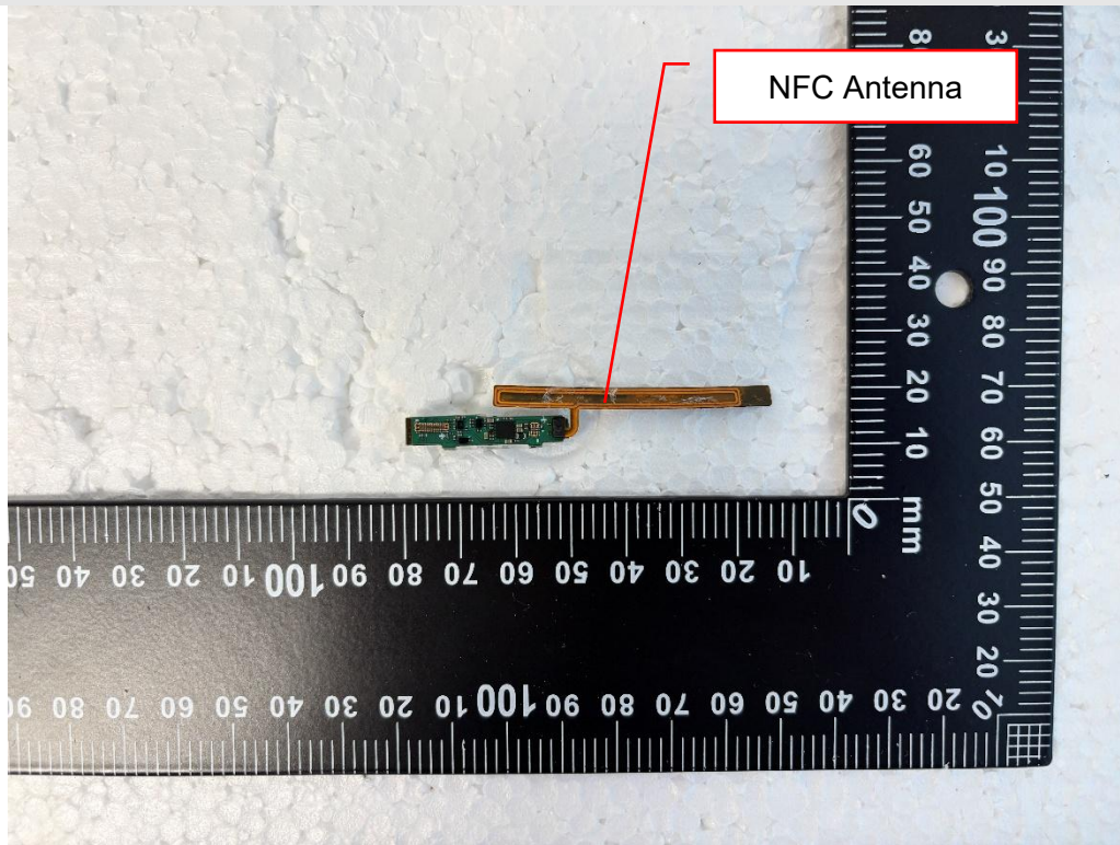
Left Frame Internal View of EUT-8
