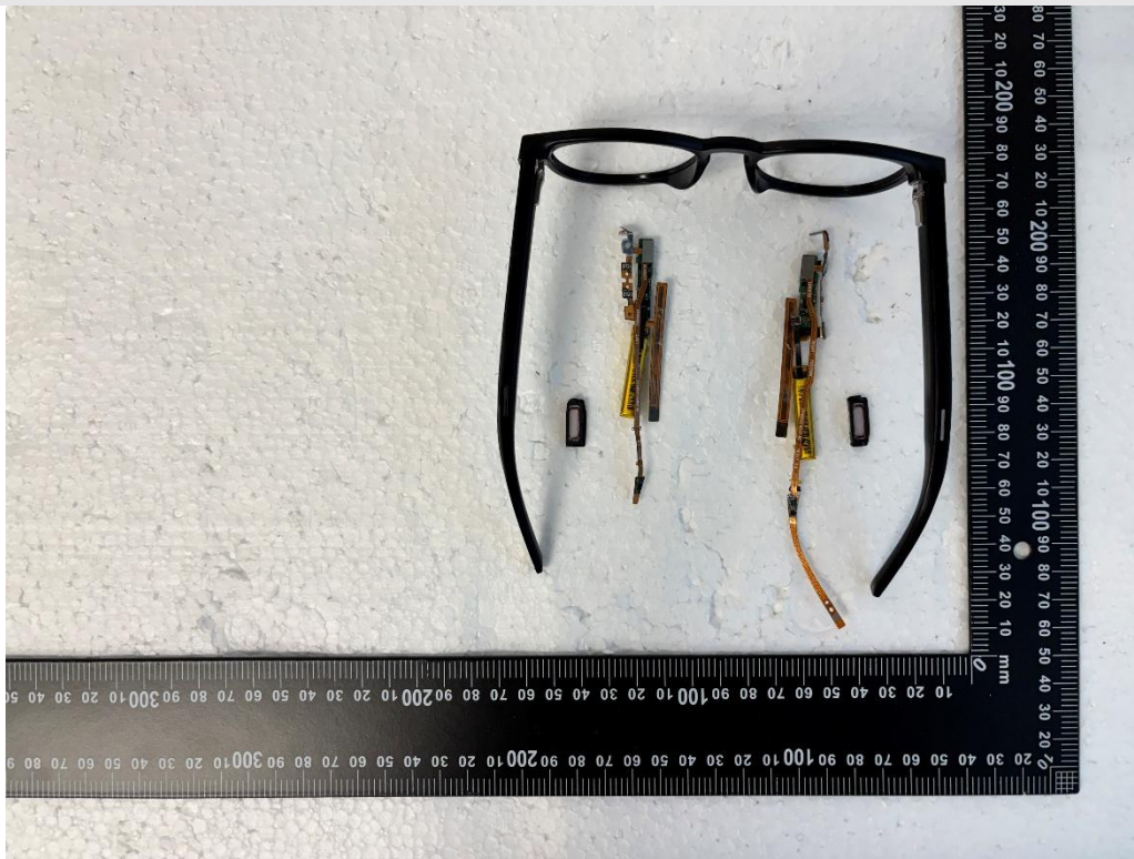
Left Frame Internal View of EUT-4
