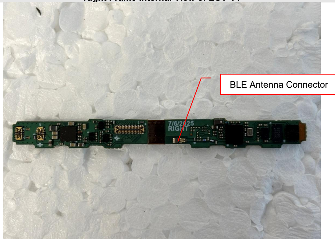
Right Frame Internal View of EUT-14
