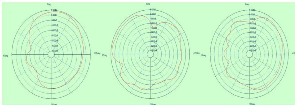
2550MHz (Phi0/Phi90/Theta90)
