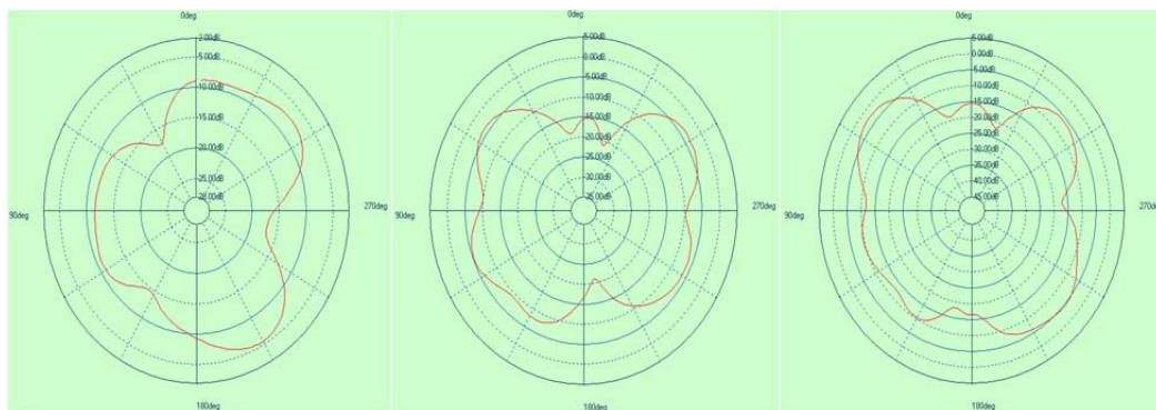
890MHz (Phi0/Phi90/Theta90)
