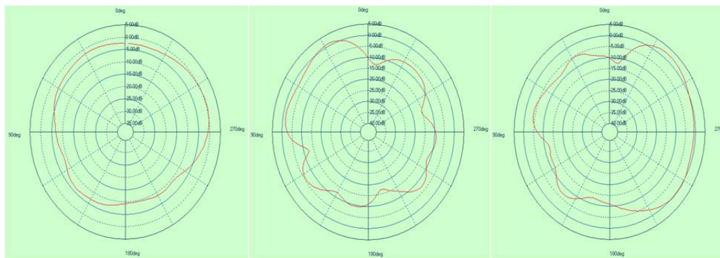
2550MHz (Phi0/Phi90/Theta90)
