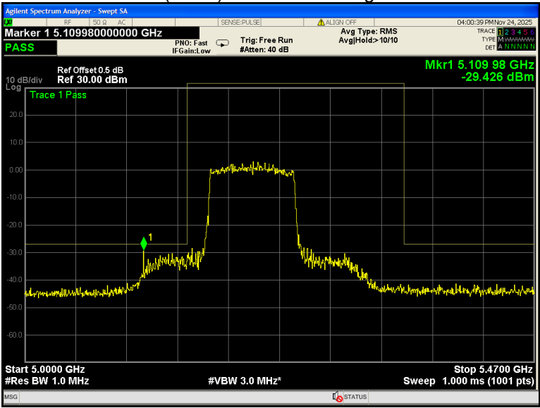
802.11ax(HE80) U-NII-1 Band edge-left side
