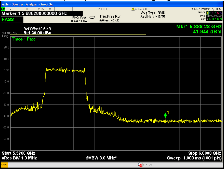
802.11ax(HE80) U-NII-2C Band edge-right side
