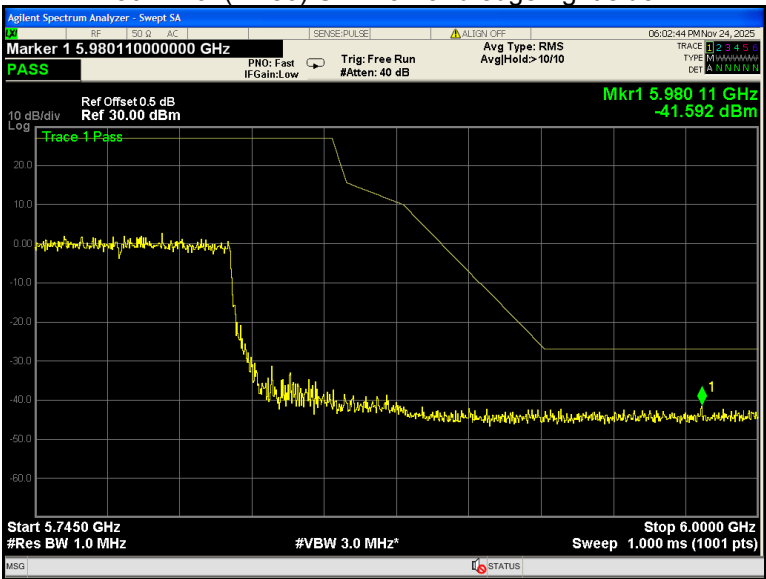
802.11ax(HE80) U-NII-3 Band edge-right side
