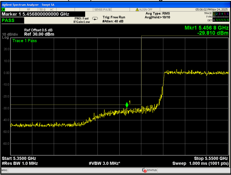
802.11ax(HE80) U-NII-2C Band edge-left side
