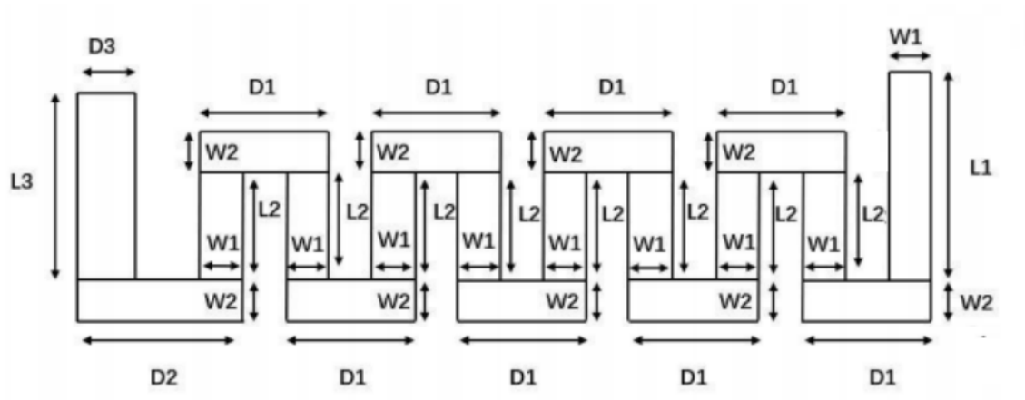
Antenna Dimensions
