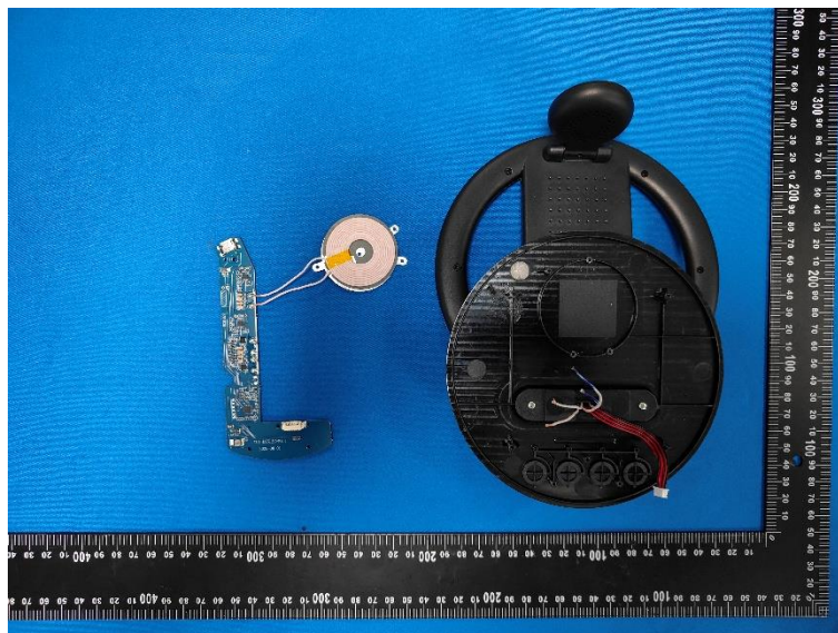
Loop Antenna
