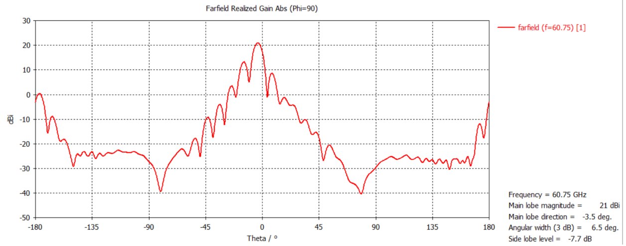
Figure 3: Antenna HPlane Gain
