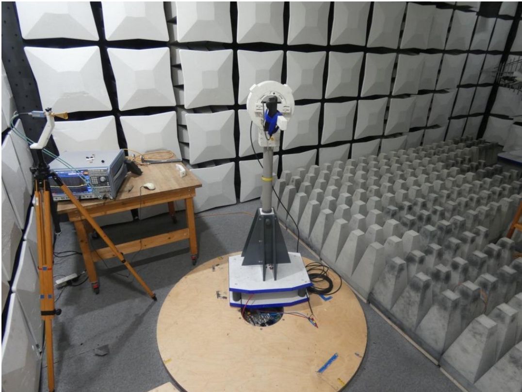
Photo 6: Test setup for radiated emissions measurements above 26 GHz in the fully anechoic room (FAR)
