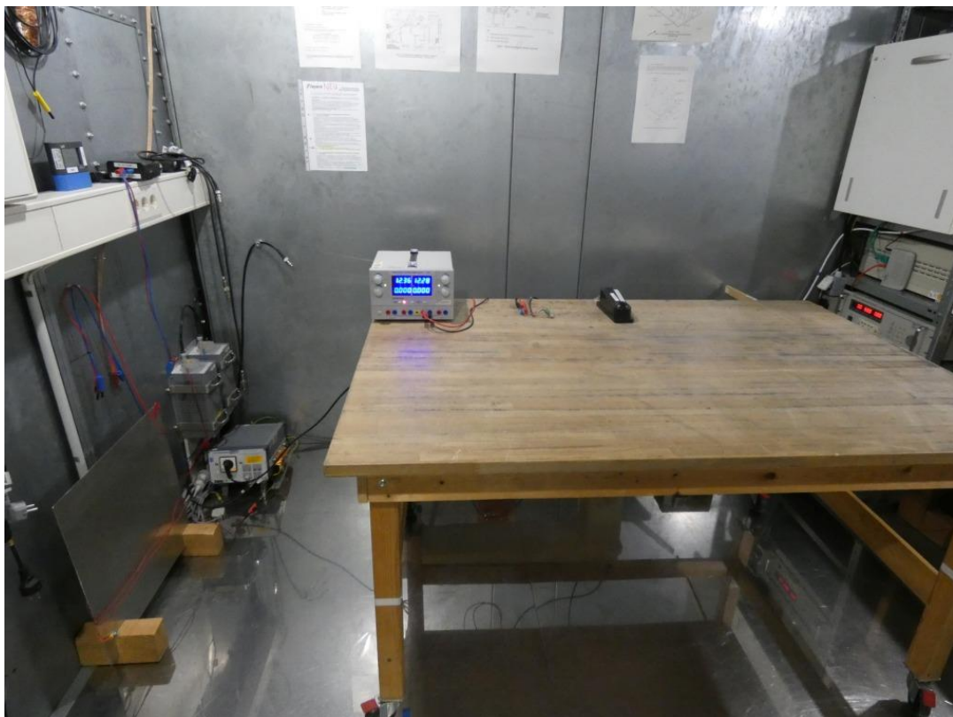
Photo 4: Test setup with Setup S01_AC01 for conducted emissions measurements below 30 MHz
