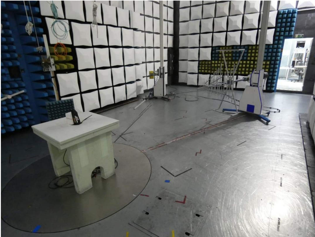
Photo 1: Test setup (stand alone setup) for radiated emissions measurements below 1 GHz in the semi anechoic room (SAR)
