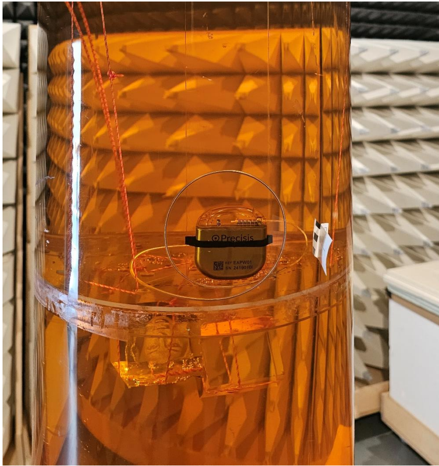
Test setup (radiated)
