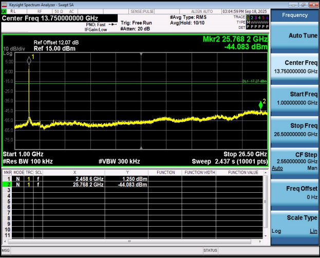
11N20SISO-Ant1-2462-1000~26500-PASS
