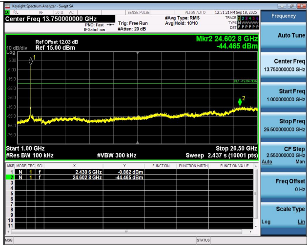
11G-Ant1-2437-1000~26500-PASS
