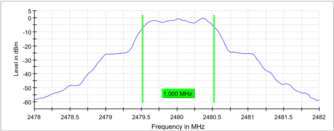
1M_HCH_2480MHz_Ant1_NTNV 6 dB Bandwidth
