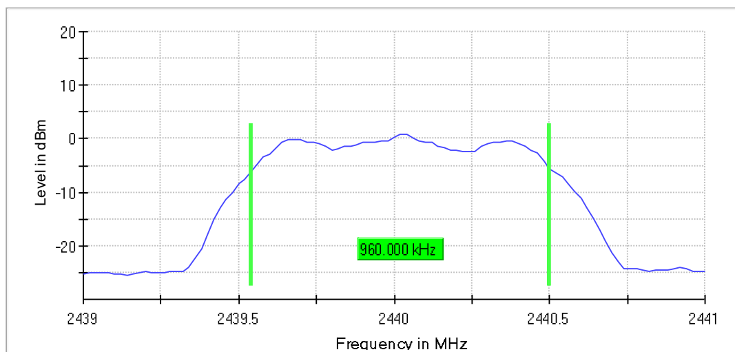
1M_MCH_2440MHz_Ant1_NTNV
