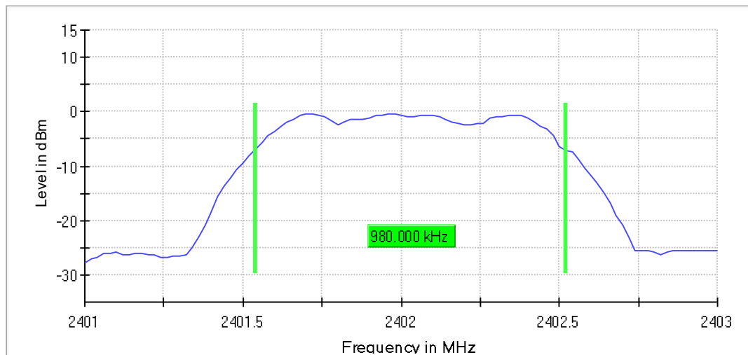
1M_LCH_2402MHz_Ant1_NTNV
