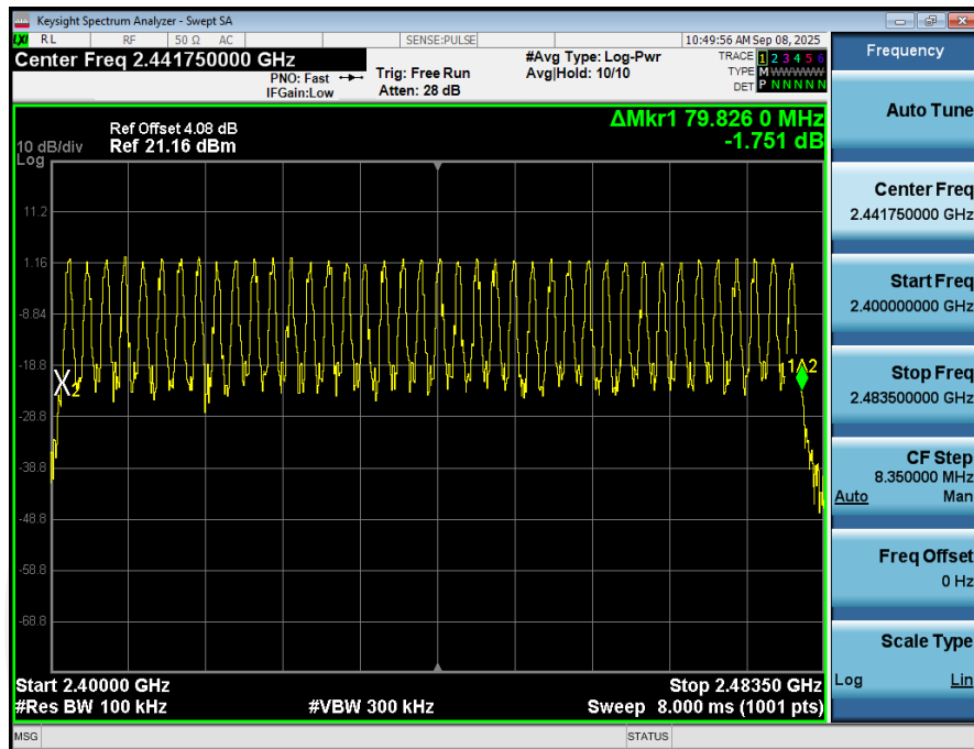
Number_of_Hopping_Channel_(Hopping)_NVNT_ANT1_GFSK_Hopping
