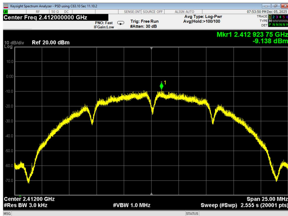
Figure 19 PSD, Low, Wifi B, Conducted
