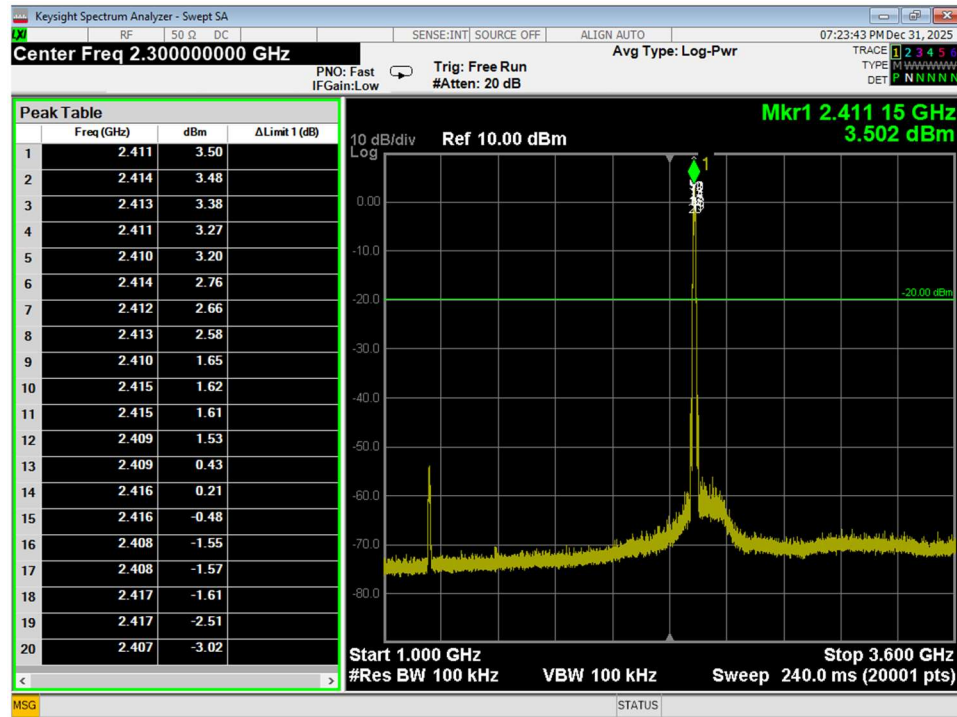
Figure 27 Conducted Spurious Emissions, Wifi B, Low Channel, Conducted, 1GHz – 3.6GHz
