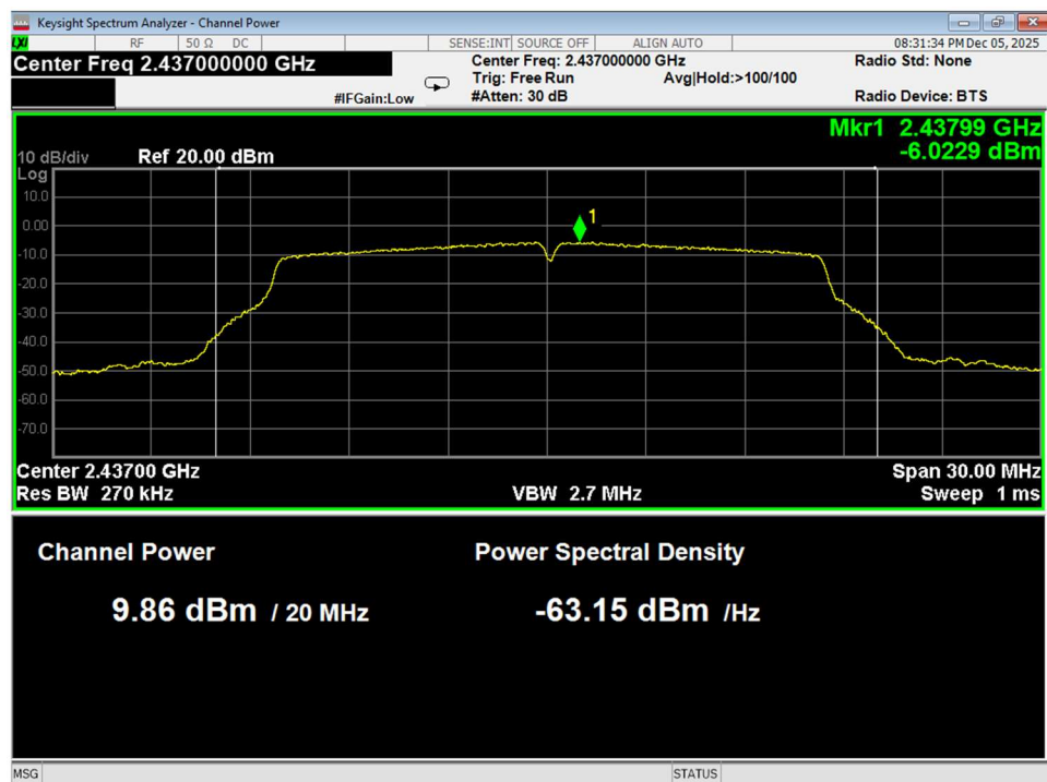
Figure 36 Average Power, Mid, Wifi G, conducted
