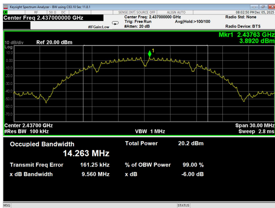
Figure 17 6dB Bandwidth, Mid, Wifi B, Conducted
