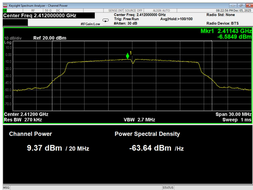
Figure 35 Average Power, Low, Wifi G, conducted
