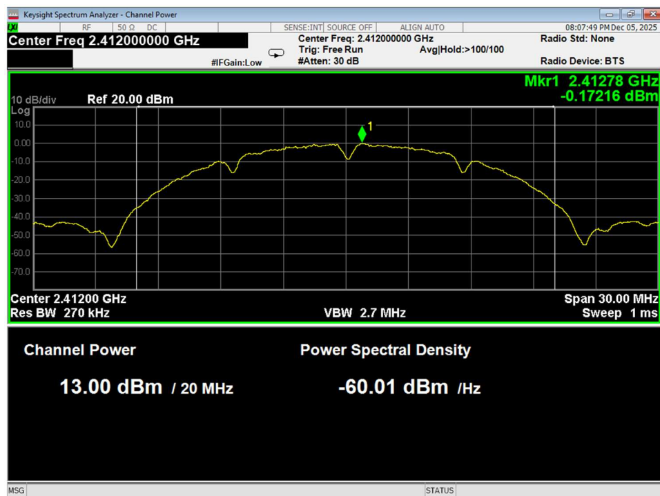
Figure 13 Average Power, Low, Wifi B, Conducted
