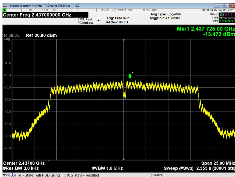
Figure 42 PSD, Mid, Wifi G, conducted
