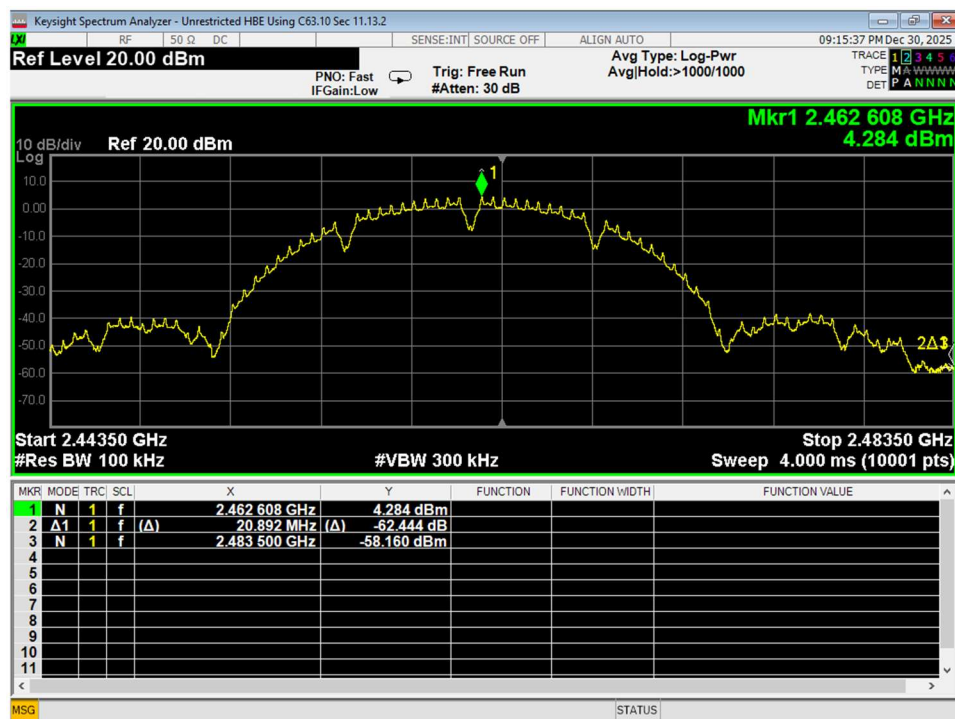
Figure 25 Upper Bandedge, Unrestricted, Wifi B, Conducted
