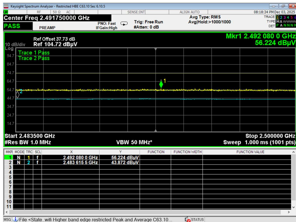
Figure 23 Upper Bandedge, Restricted, Wifi B, radiated
