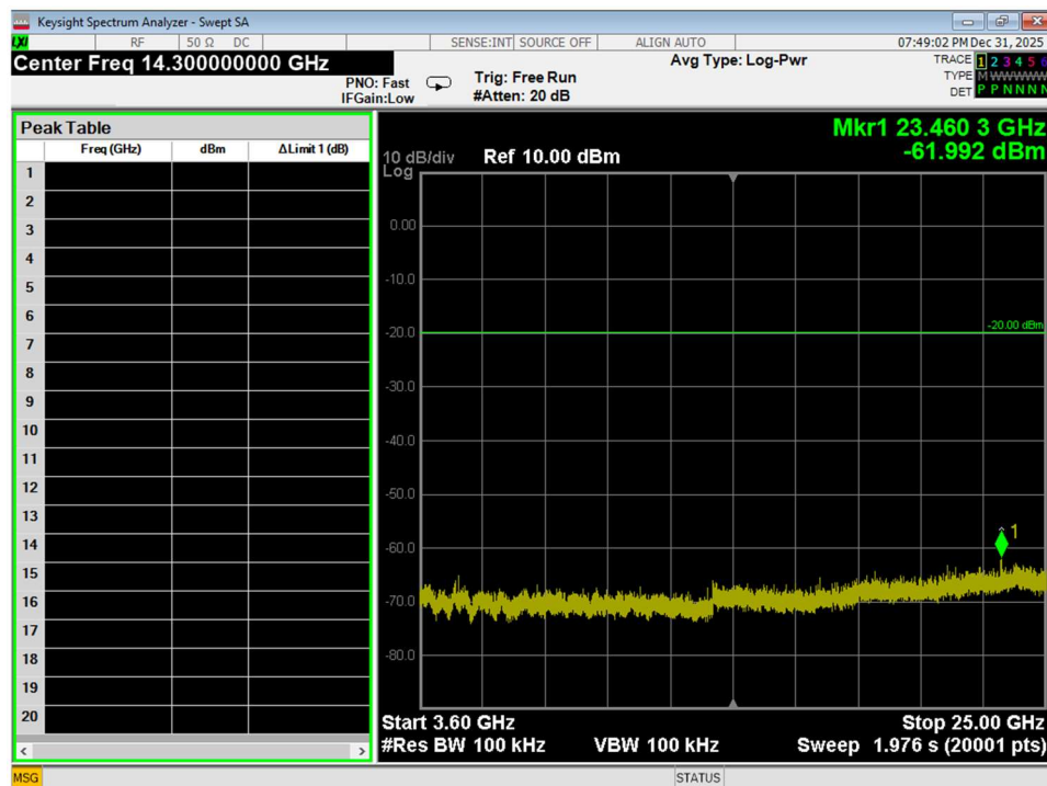
Figure 34 Conducted Spurious Emissions, Wifi B, High Channel, Conducted, 3.6GHz – 25GHz
