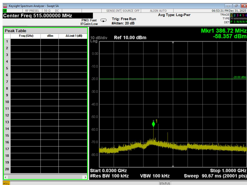
Figure 26 Conducted Spurious Emissions, Wifi B, Low Channel, Conducted, 30MHz – 1GHz
