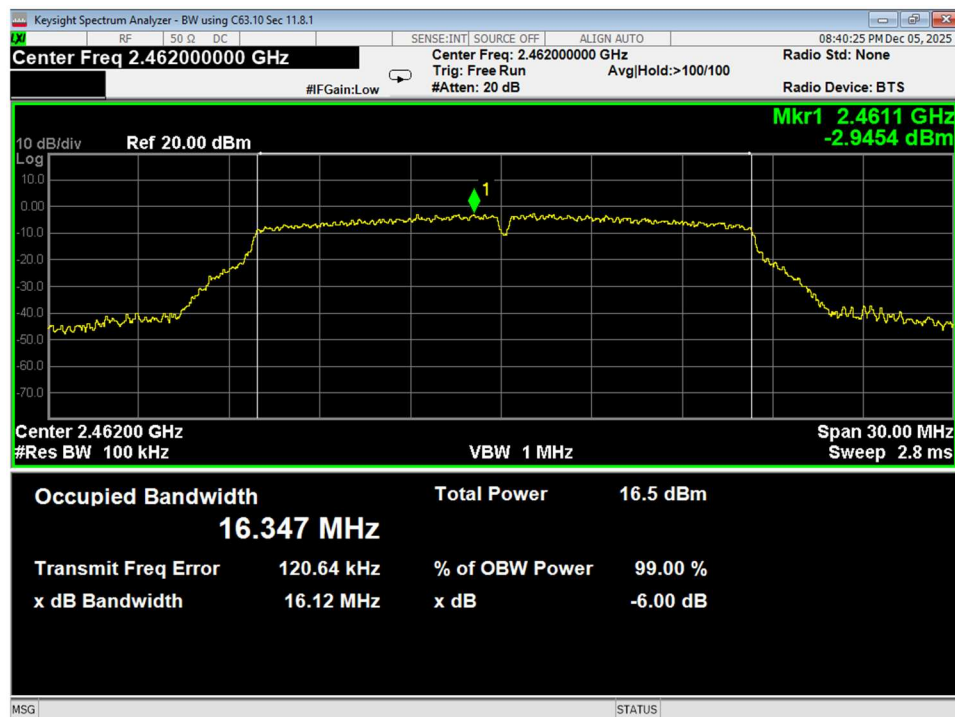
Figure 40 6dB Bandwidth, High, Wifi G, conducted
