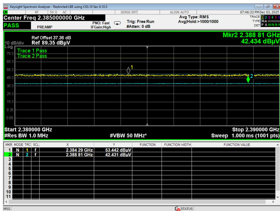
Figure 22 Lower Bandedge, Restricted, Wifi B, radiated
