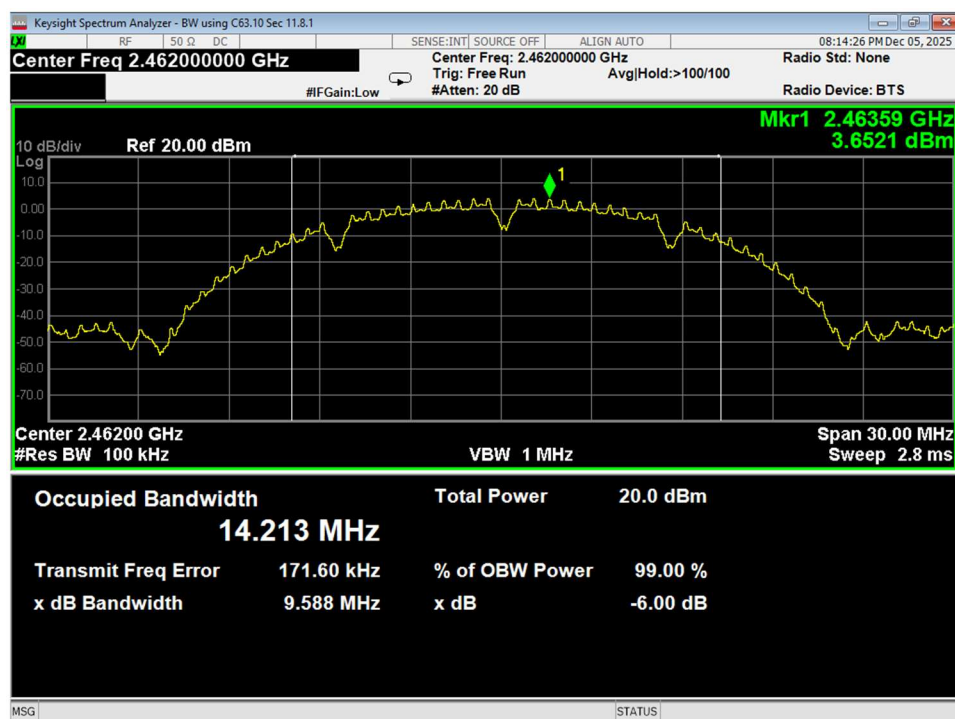
Figure 18 6dB Bandwidth, High, Wifi B, Conducted
