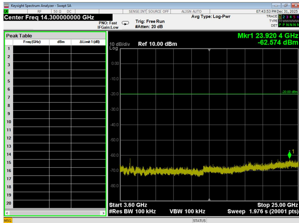
Figure 28 Conducted Spurious Emissions, Wifi B, Low Channel, Conducted, 3.6GHz – 25GHz
