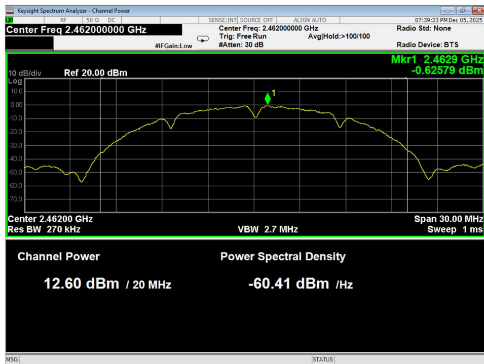
Figure 15 Average Power, High, Wifi B, Conducted
