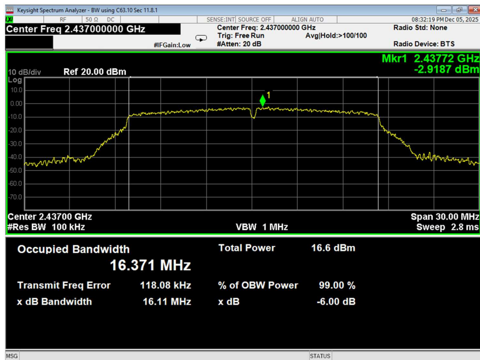
Figure 39 6dB Bandwidth, Mid, Wifi G, conducted
