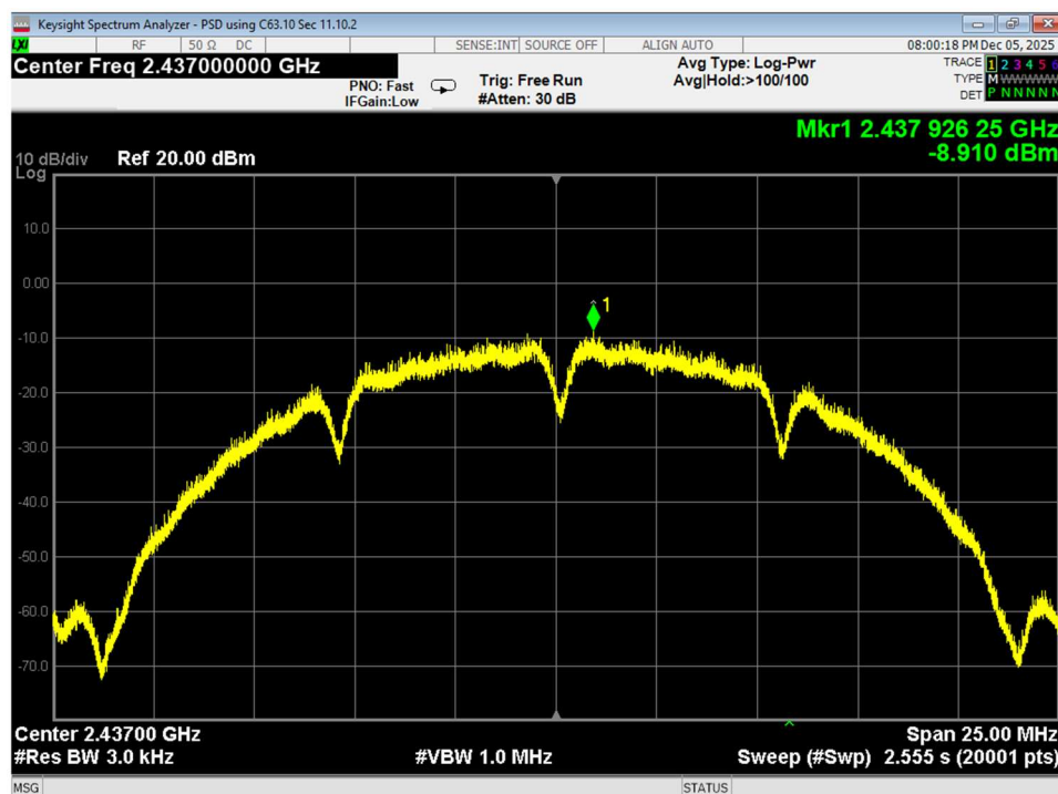
Figure 20 PSD, Mid, Wifi B, Conducted
