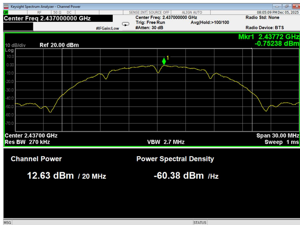
Figure 14 Average Power, Mid, Wifi B, Conducted
