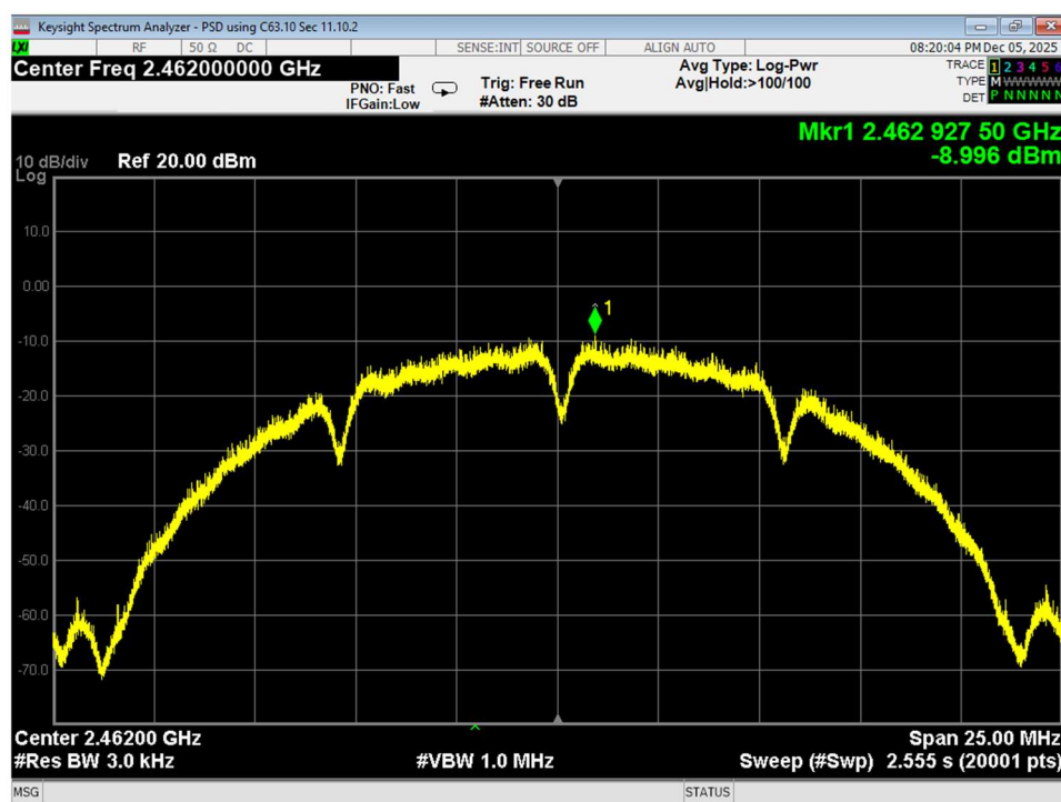
Figure 21 PSD, High, Wifi B, Conducted
