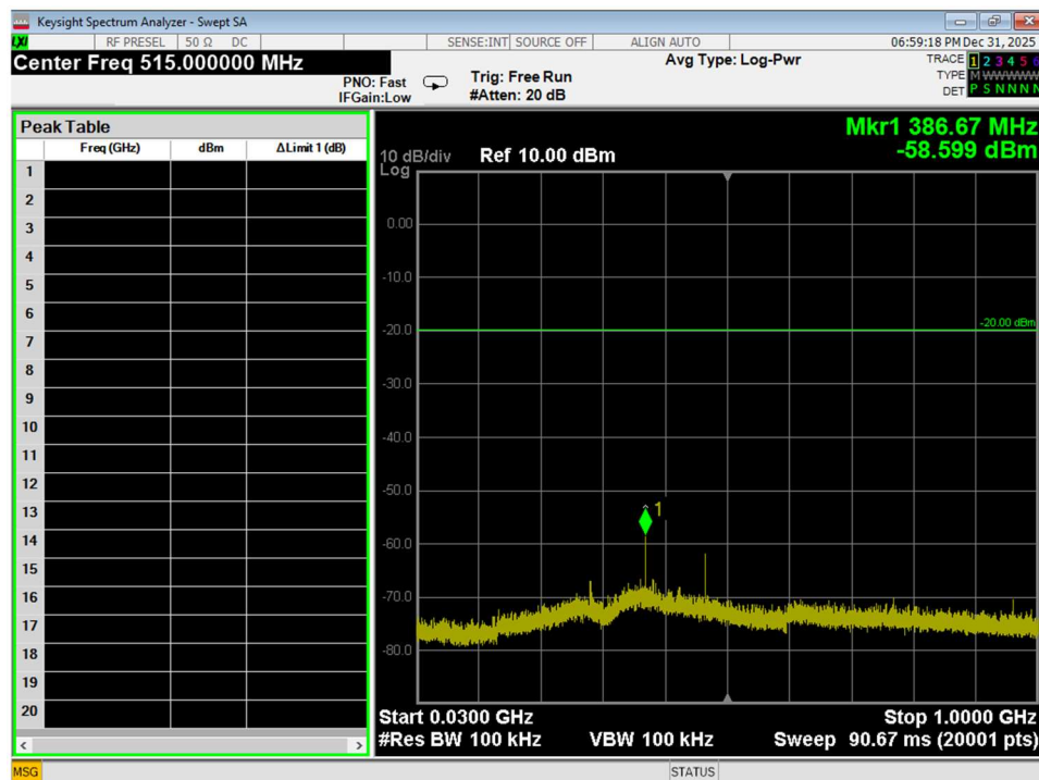
Figure 32 Conducted Spurious Emissions, Wifi B, High Channel, Conducted, 30MHz - 1GHz
