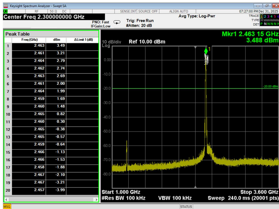
Figure 33 Conducted Spurious Emissions, Wifi B, High Channel, Conducted, 1GHz – 3.6GHz
