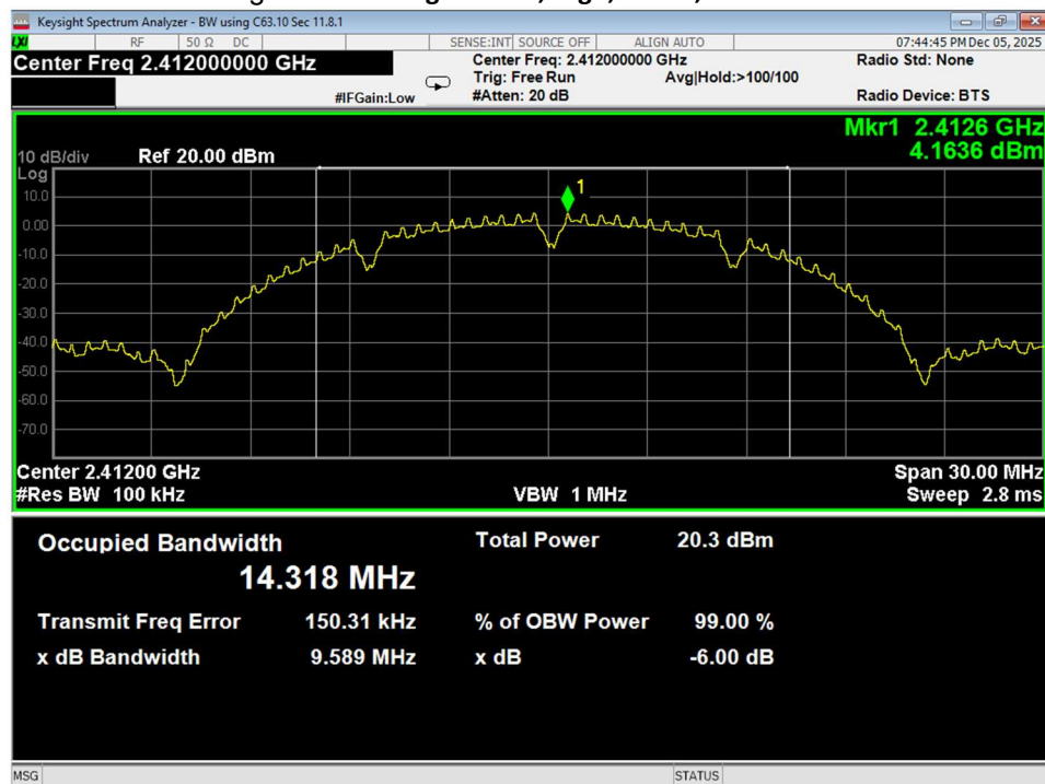
Figure 16 6dB Bandwidth, Low, Wifi B, Conducted
