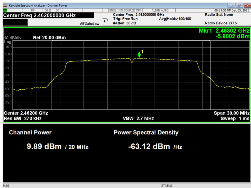
Figure 37 Average Power, High, Wifi G, conducted
