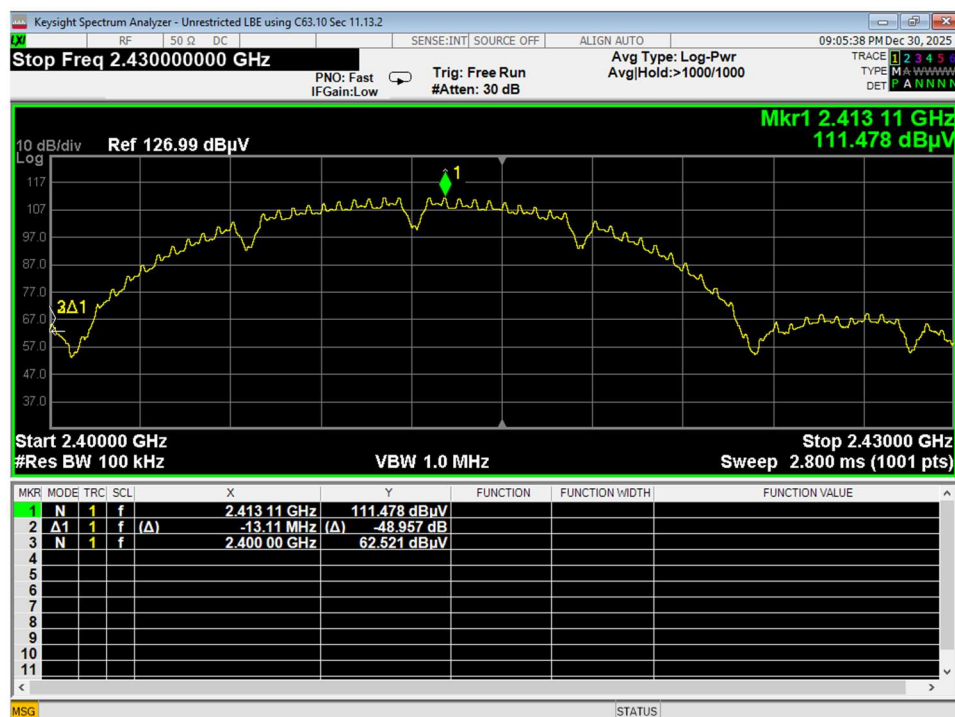
Figure 24 Lower Bandedge, Unrestricted, Wifi B, Conducted
