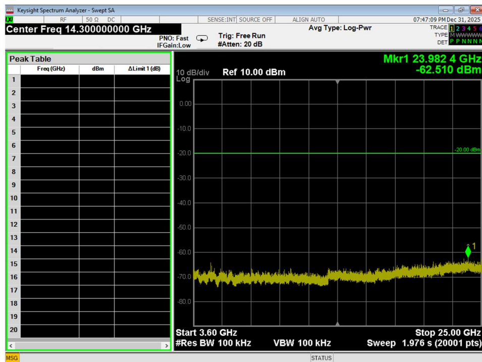
Figure 31 Conducted Spurious Emissions, Wifi B, Mid Channel, Conducted, 3.6GHz – 25GHz
