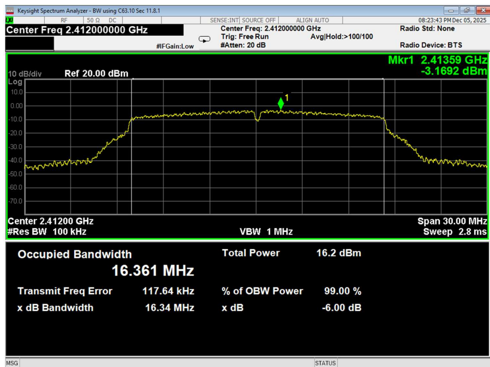
Figure 38 6dB Bandwidth, Low, Wifi G, conducted
