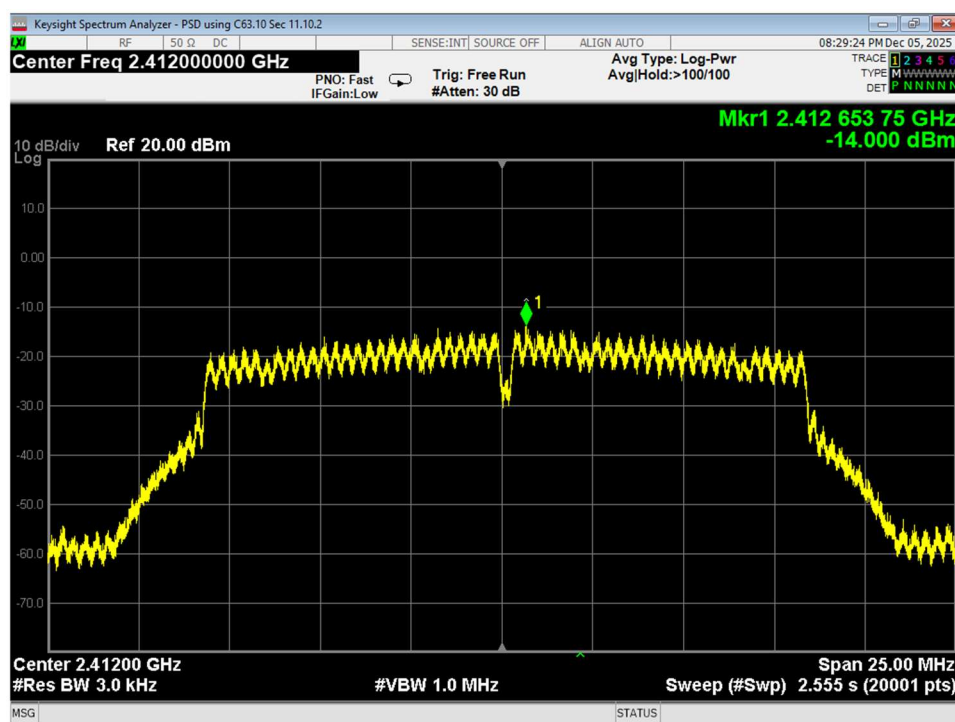
Figure 41 PSD, Low, Wifi G, conducted
