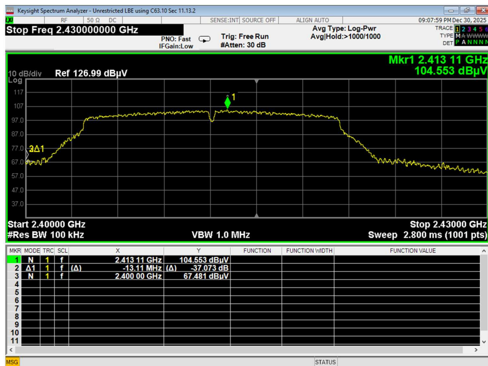
Figure 46 Lower Bandedge, Unrestricted, Wifi G, conducted
