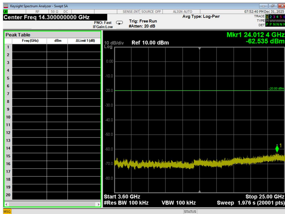
Figure 53 Conducted Spurious Emissions, Wifi G, Mid Channel, conducted, 3.6GHz – 25GHz
