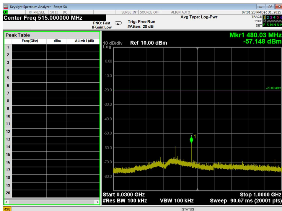
Figure 48 Conducted Spurious Emissions, Wifi G, Low Channel, conducted, 30MHz – 1GHz
