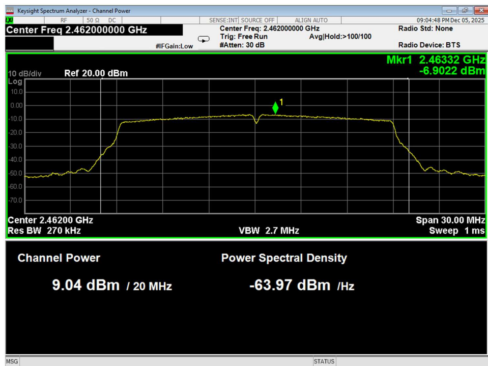
Figure 59 Average Power, High, Wifi N, conducted
