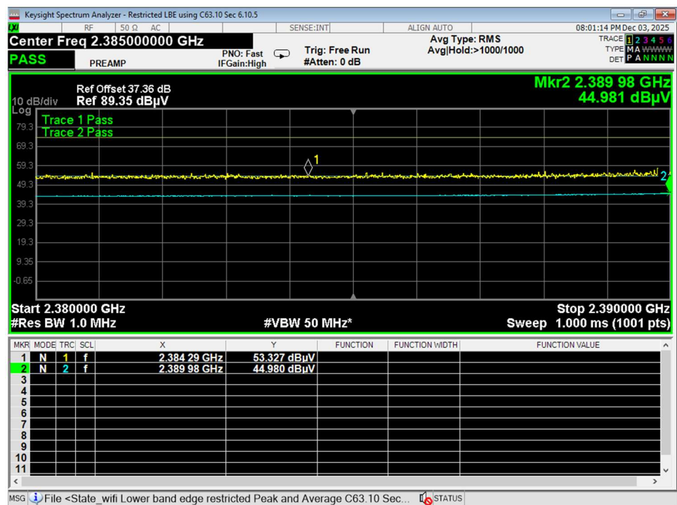
Figure 66 Lower Bandedge, Restricted, Wifi N, radiated
