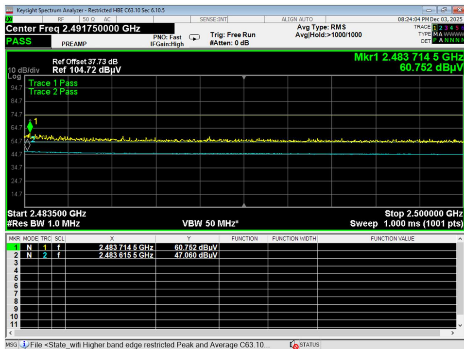
Figure 45 Higher Bandedge, Restricted, Wifi G, radiated
