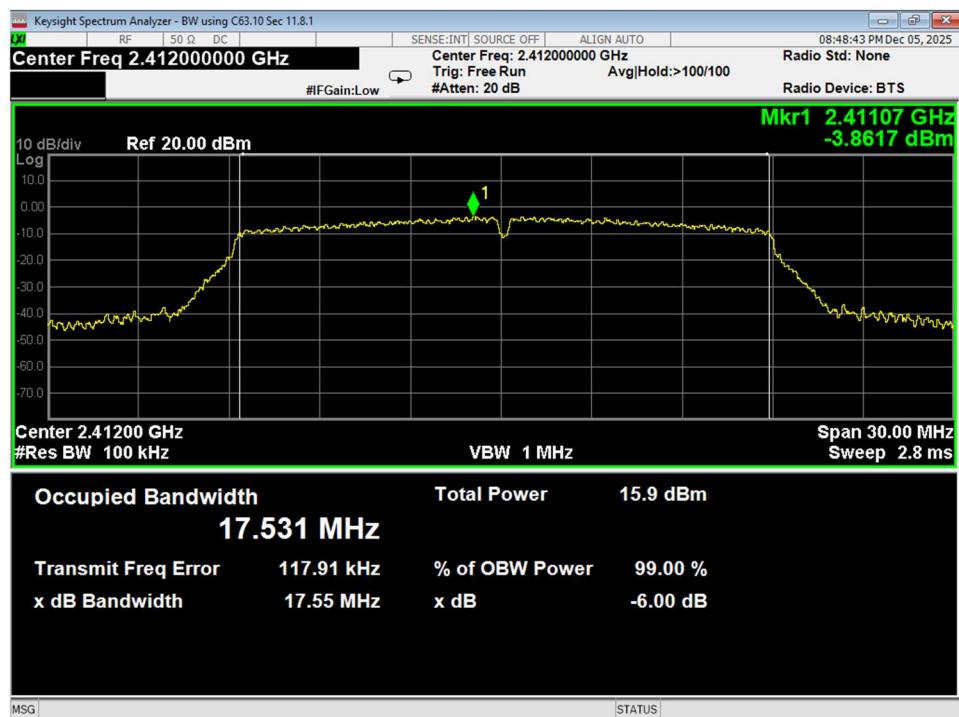
Figure 60 6dB Bandwidth, Low, Wifi N, conducted
