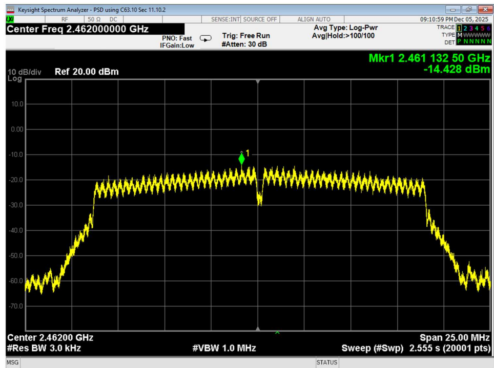
Figure 65 PSD, High, Wifi N, conducted
