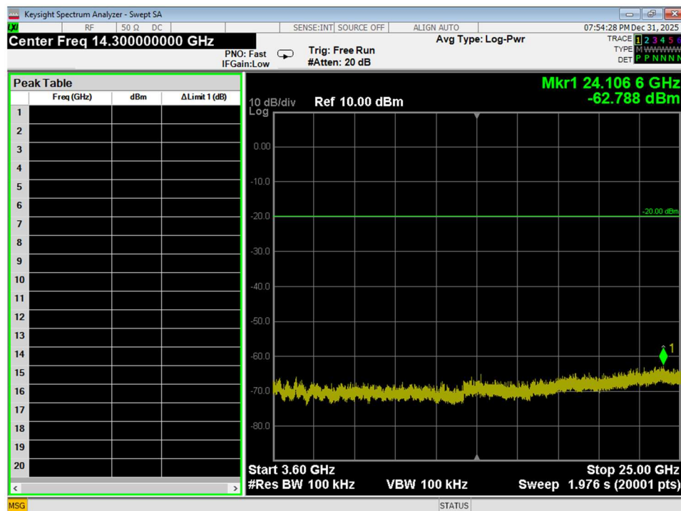
Figure 56 Conducted Spurious Emissions, Wifi G, High Channel, conducted, 3.6GHz – 25GHz
