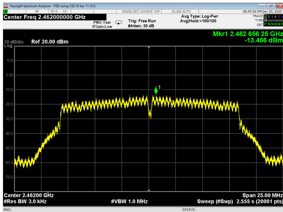
Figure 43 PSD, High, Wifi G, conducted
