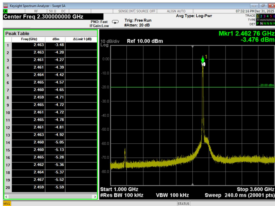
Figure 55 Conducted Spurious Emissions, Wifi G, High Channel, conducted, 1GHz – 3.6GHz
