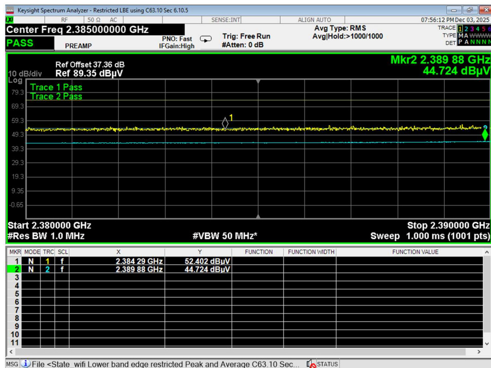
Figure 44 Lower Bandedge, Restricted, Wifi G, radiated
