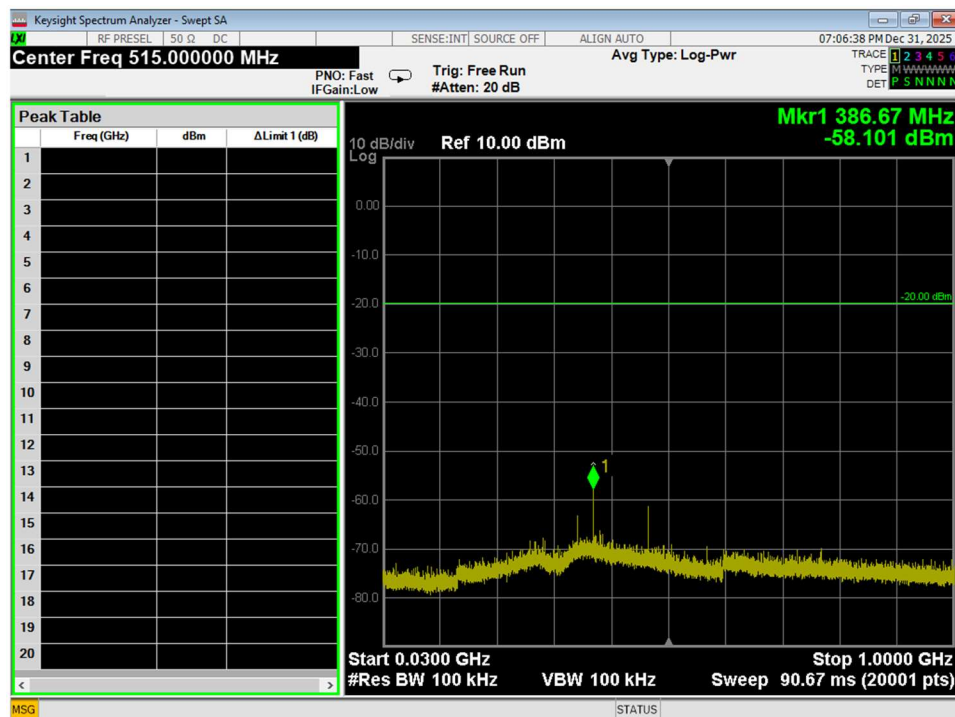
Figure 54 Conducted Spurious Emissions, Wifi G, High Channel, conducted, 30MHz - 1GHz
