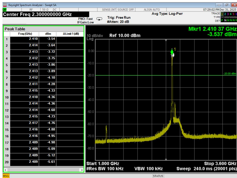
Figure 49 Conducted Spurious Emissions, Wifi G, Low Channel, conducted, 1GHz – 3.6GHz
