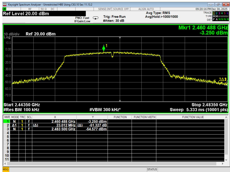
Figure 69 Higher Bandedge, Unrestricted, Wifi N, conducted
