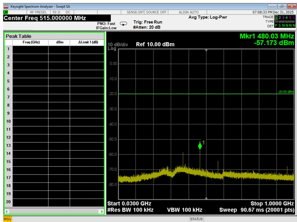
Figure 70 Conducted Spurious Emissions, Wifi N, Low Channel, conducted, 30MHz - 1GHz
