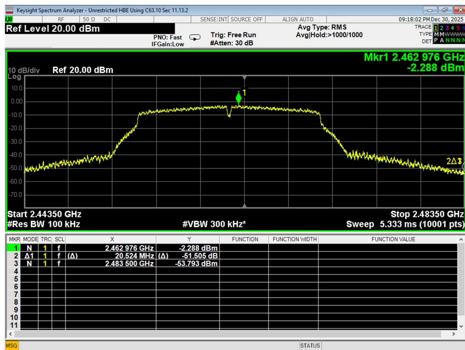
Figure 47 Higher Bandedge, Unrestricted, Wifi G, conducted
