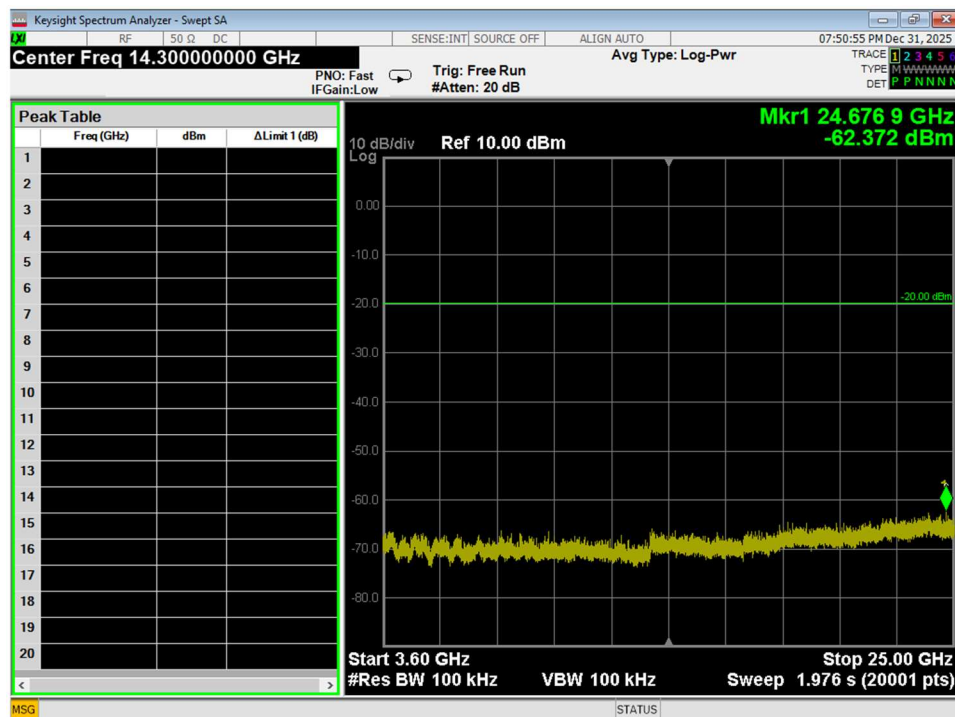
Figure 50 Conducted Spurious Emissions, Wifi G, Low Channel, conducted, 3.6GHz – 25GHz
