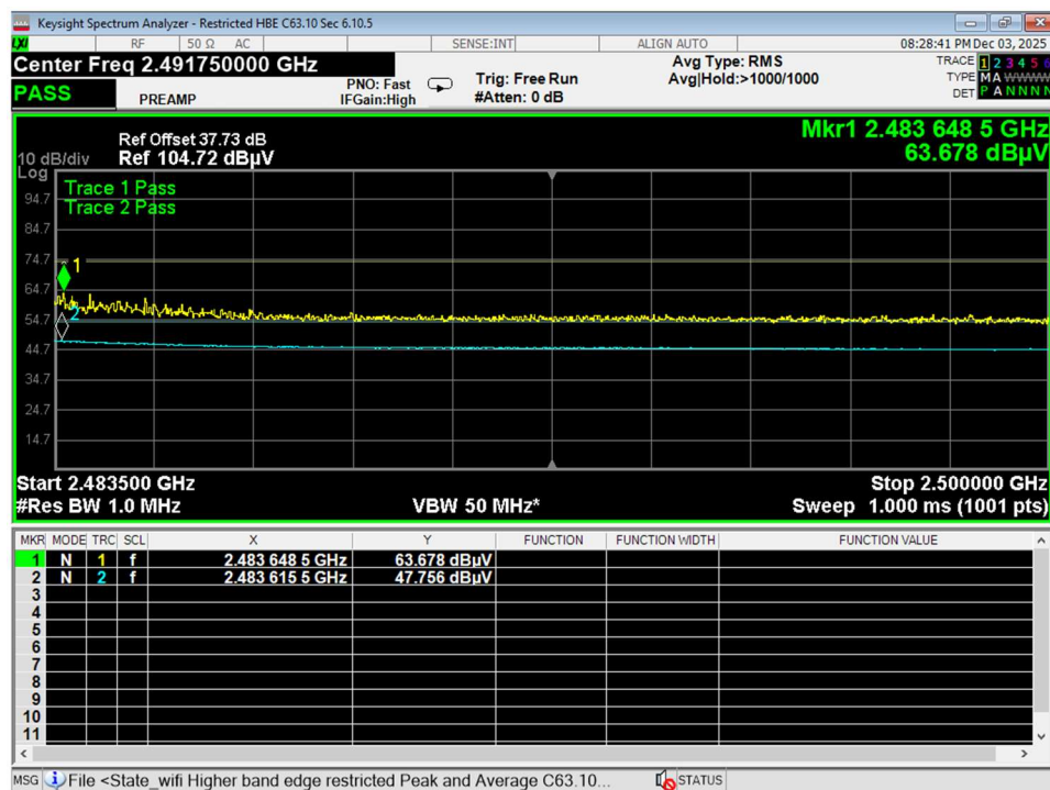
Figure 67 Higher Bandedge, Restricted, Wifi N, radiated
