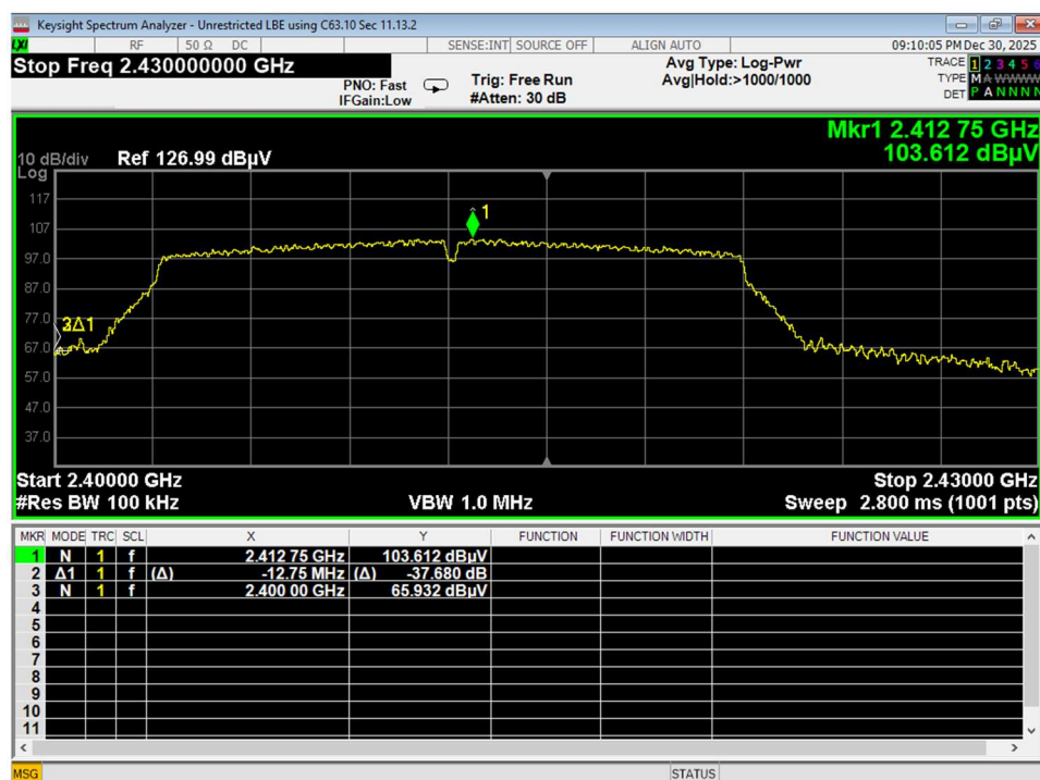
Figure 68 Lower Bandedge, Unrestricted, Wifi N, conducted
