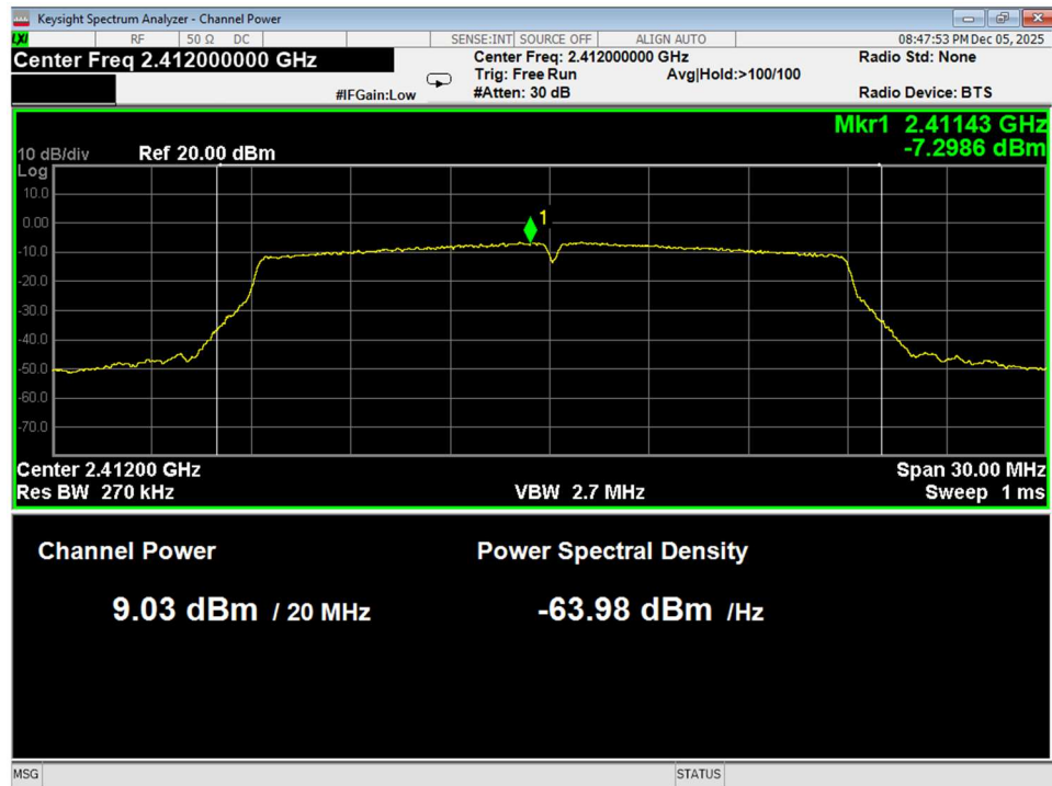
Figure 57 Average Power, Low, Wifi N, conducted
