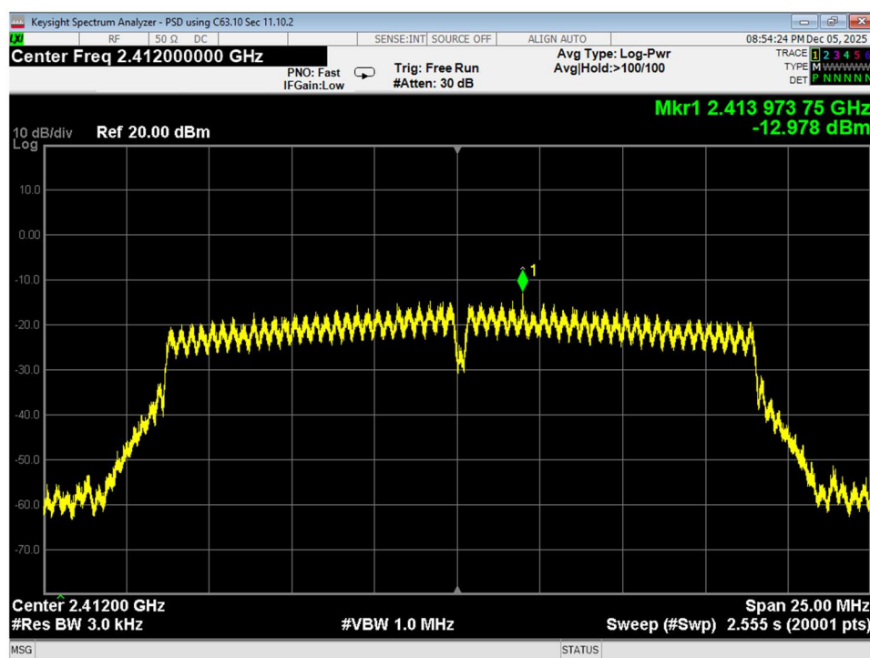
Figure 63 PSD, Low, Wifi N, conducted
