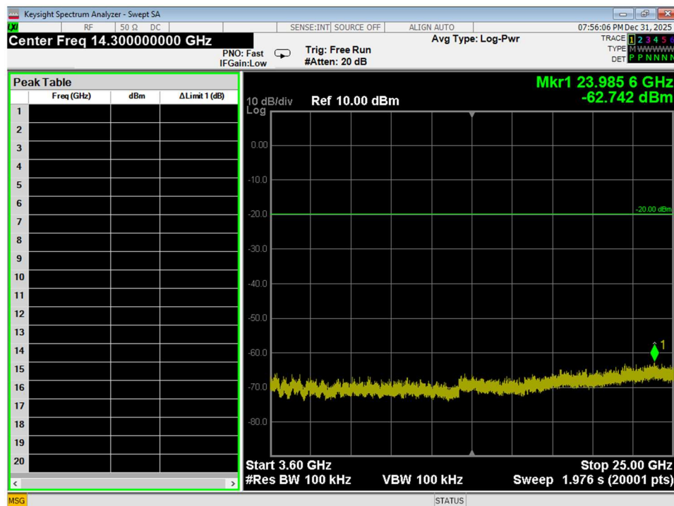
Figure 72 Conducted Spurious Emissions, Wifi N, Low Channel, conducted, 3.6GHz – 25GHz
