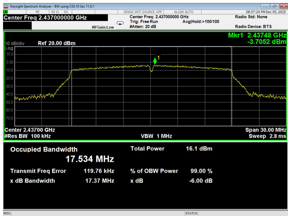
Figure 61 6dB Bandwidth, Mid, Wifi N, conducted
