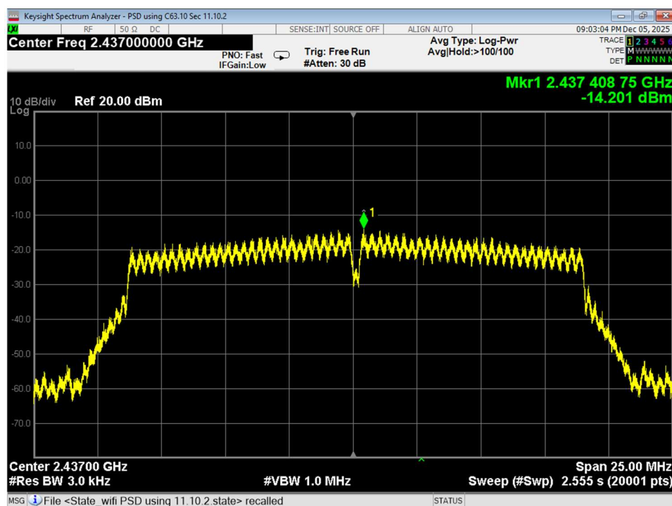
Figure 64 PSD, Mid, Wifi N, conducted
