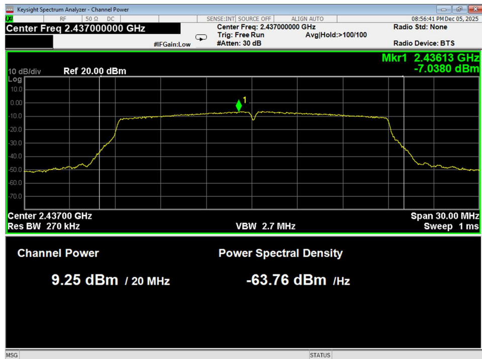
Figure 58 Average Power, Mid, Wifi N, conducted
