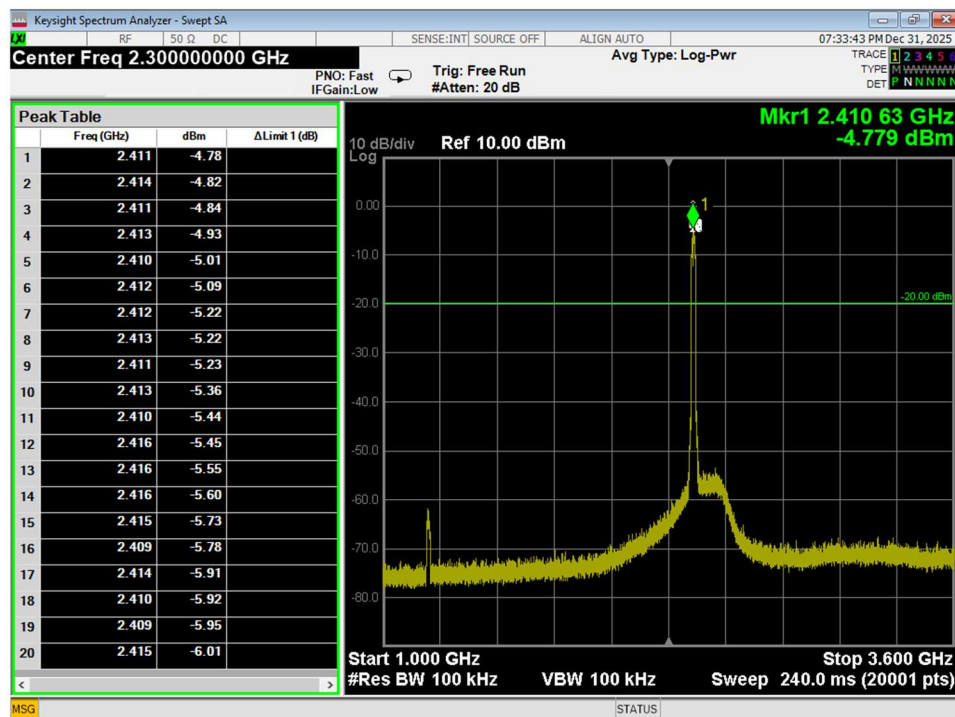
Figure 71 Conducted Spurious Emissions, Wifi N, Low Channel, conducted, 1GHz – 3.6GHz
