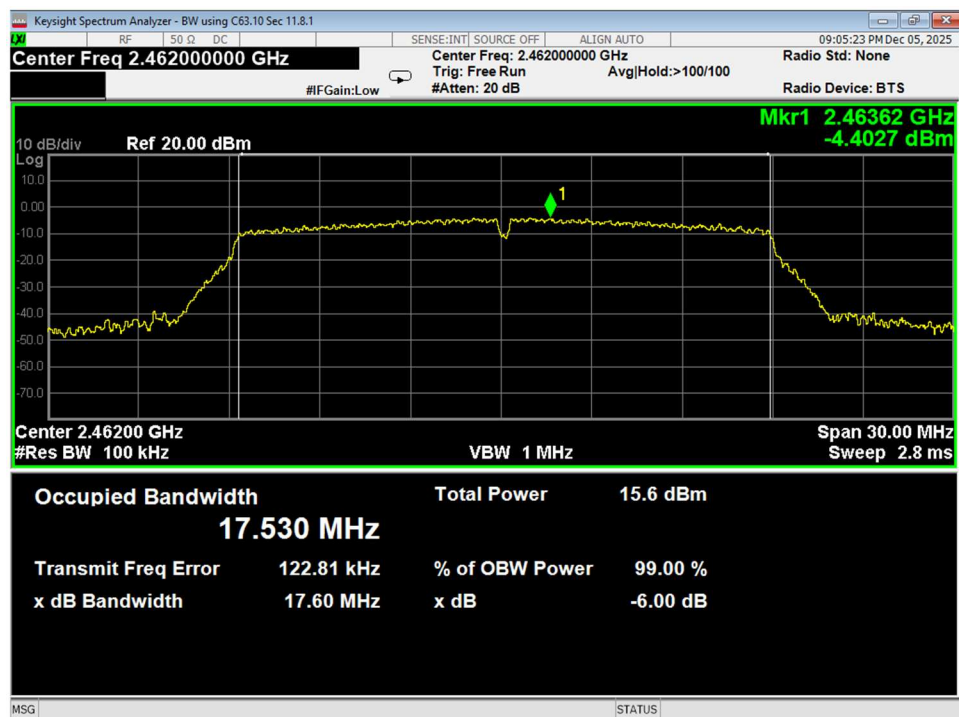
Figure 62 6dB Bandwidth, High, Wifi N, conducted
