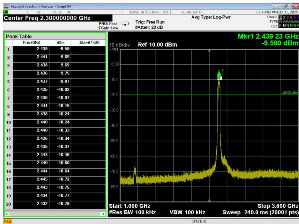
Figure 96 Conducted Spurious Emissions, Wifi N, 40MHz Bandwidth, Mid Channel, conducted, 1GHz – 3.6GHz
