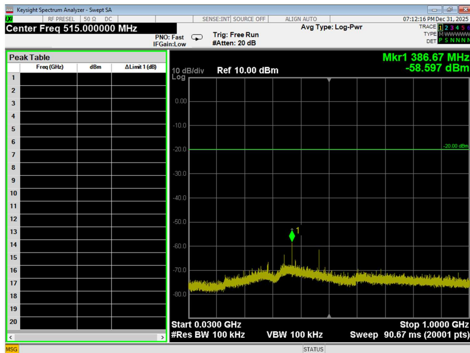
Figure 76 Conducted Spurious Emissions, Wifi N, High Channel, conducted, 30MHz – 1GHz
