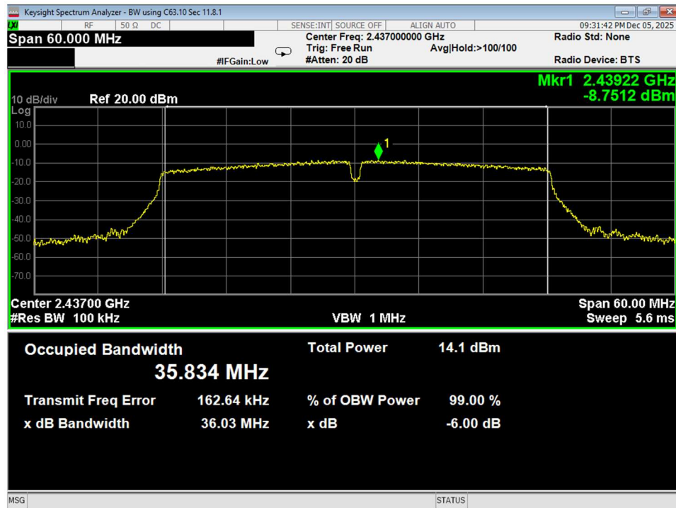
Figure 83 6dB Bandwidth, Mid, Wifi N, 40MHz bandwidth, conducted
