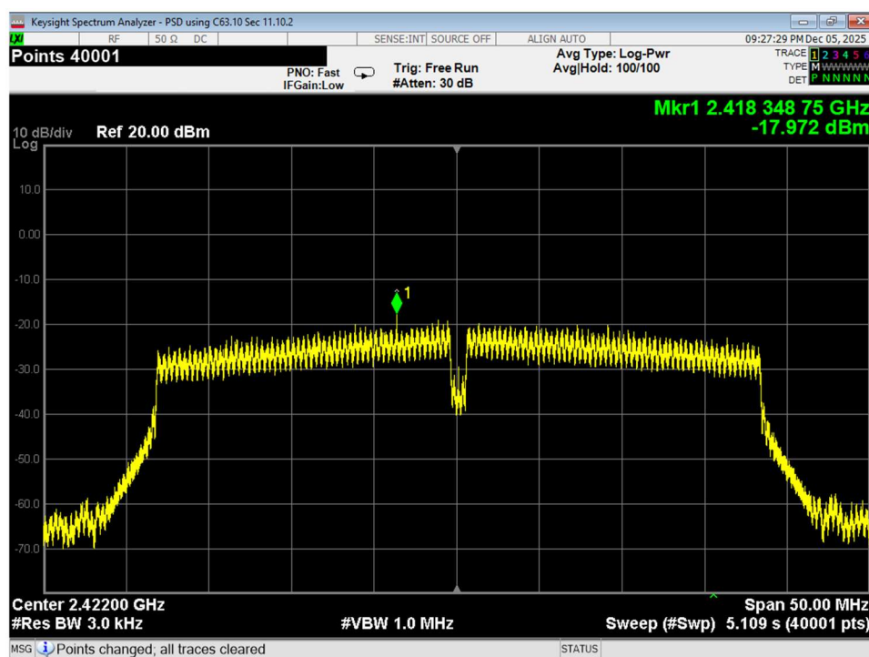
Figure 85 PSD, Low, Wifi N, 40MHz bandwidth, conducted
