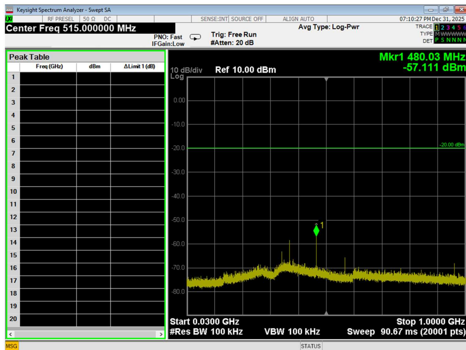
Figure 73 Conducted Spurious Emissions, Wifi N, Mid Channel, conducted, 30MHz – 1GHz
