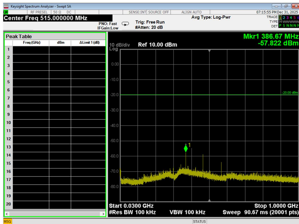
Figure 95 Conducted Spurious Emissions, Wifi N, 40MHz Bandwidth, Mid Channel, conducted, 30MHz – 1GHz
