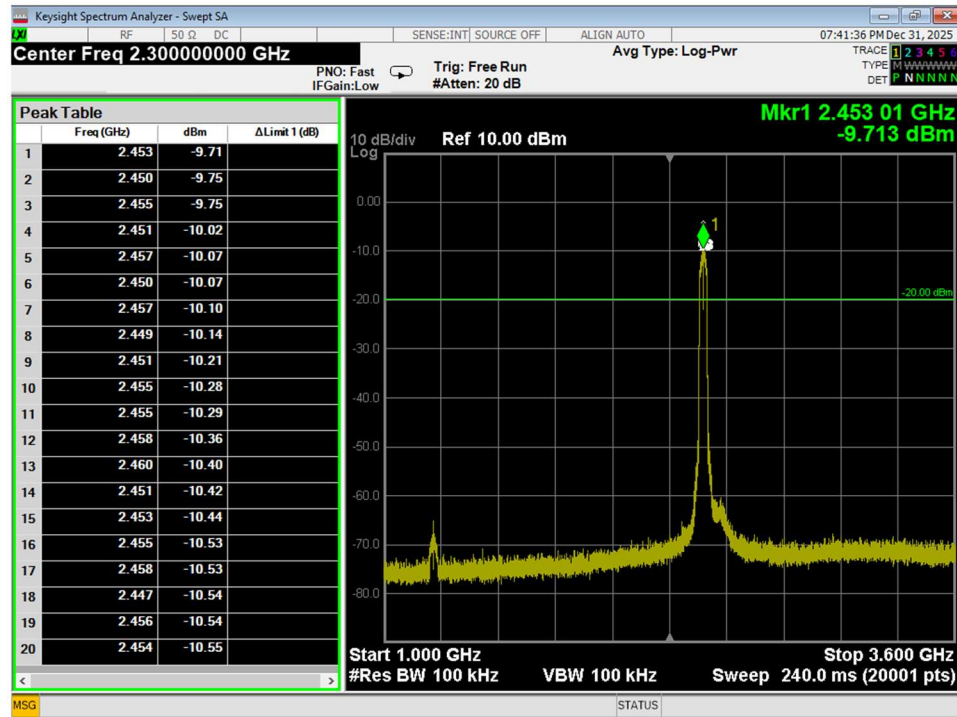
Figure 99 Conducted Spurious Emissions, Wifi N, 40MHz Bandwidth, High Channel, conducted, 1GHz – 3.6GHz
