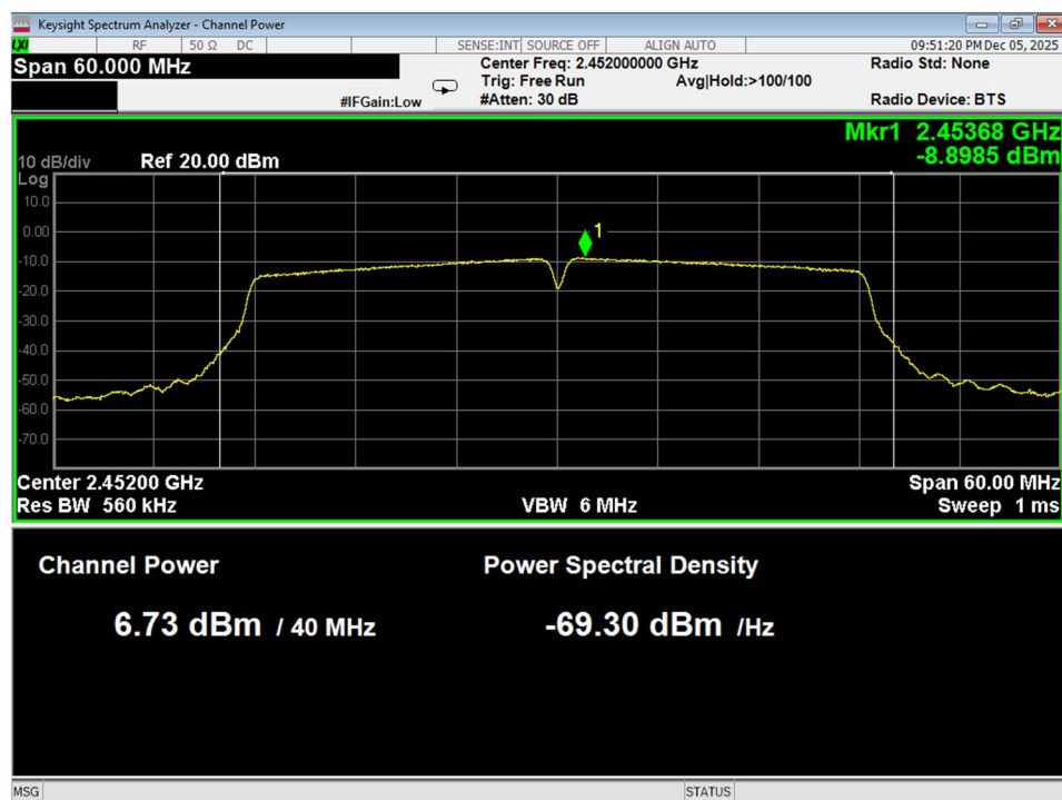
Figure 81 Average Power, High, Wifi N, 40MHz bandwidth, conducted
