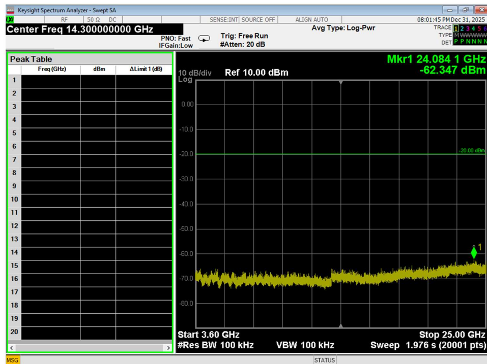
Figure 94 Conducted Spurious Emissions, Wifi N, 40MHz Bandwidth, Low Channel, conducted, 3.6GHz – 25GHz
