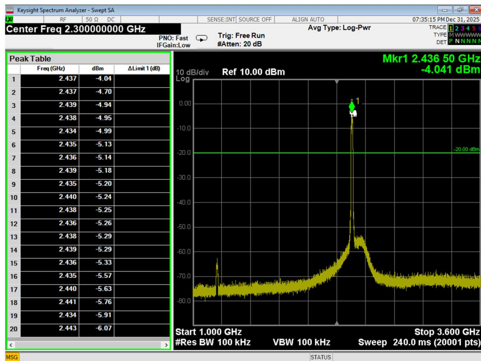
Figure 74 Conducted Spurious Emissions, Wifi N, Mid Channel, conducted, 1GHz – 3.6GHz
