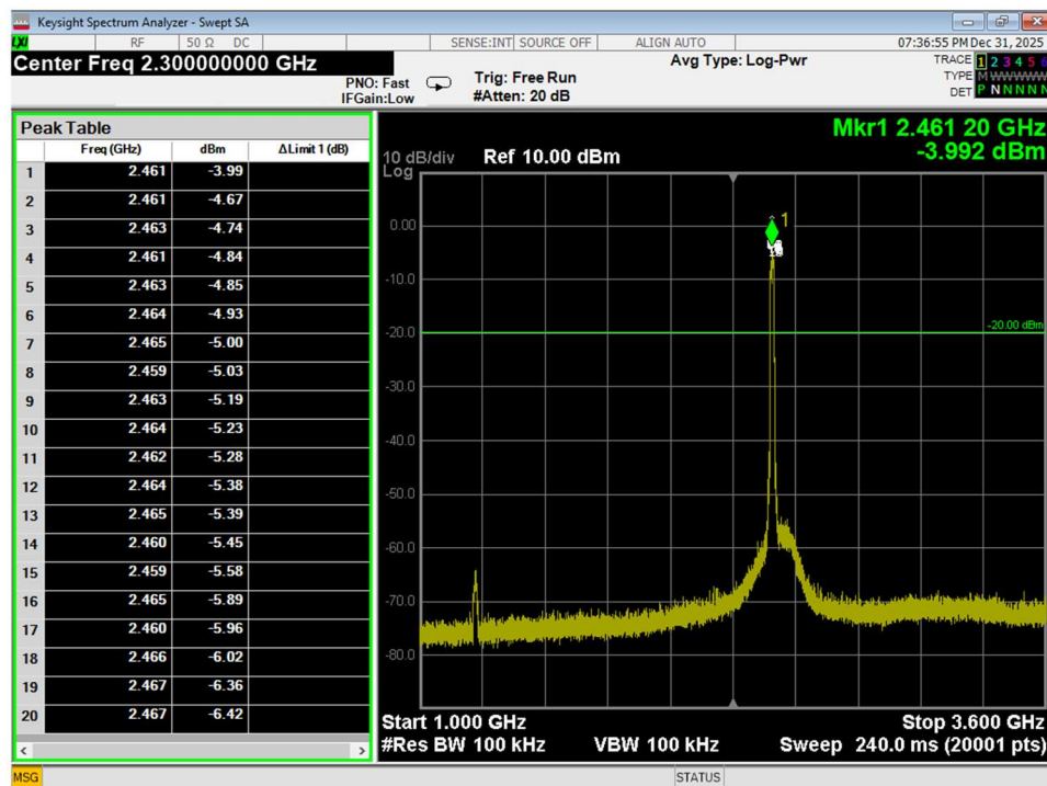
Figure 77 Conducted Spurious Emissions, Wifi N, High Channel, conducted, 1GHz – 3.6GHz
