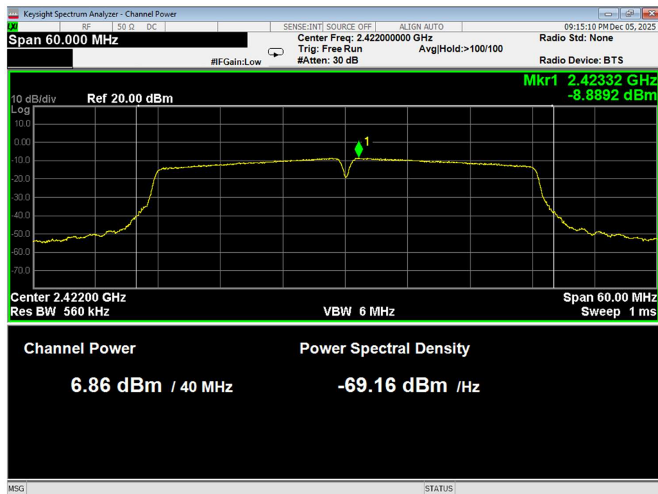
Figure 79 Average Power, Low, Wifi N, 40MHz bandwidth, conducted
