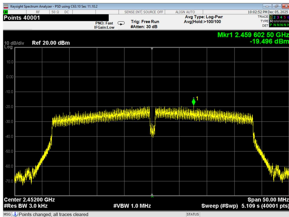
Figure 87 PSD, High, Wifi N, 40MHz bandwidth, conducted
