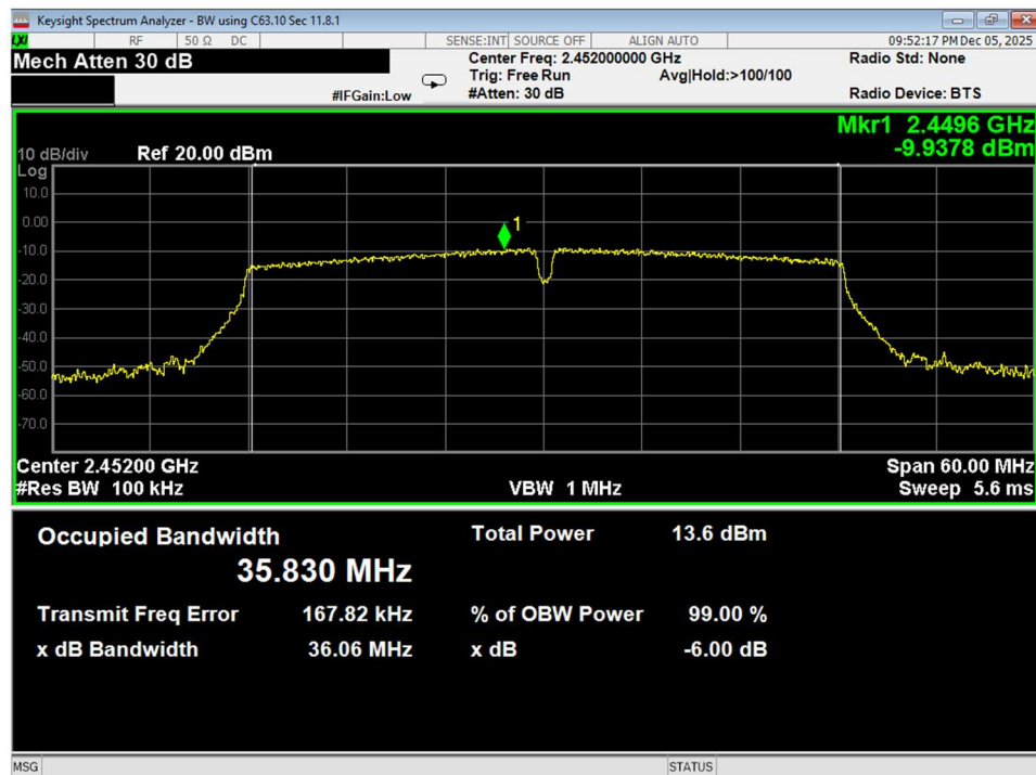
Figure 84 6dB Bandwidth, High, Wifi N, 40MHz bandwidth, conducted
