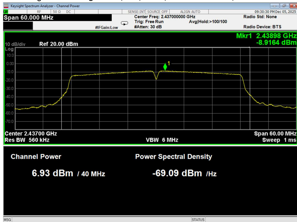
Figure 80 Average Power, Mid, Wifi N, 40MHz bandwidth, conducted
