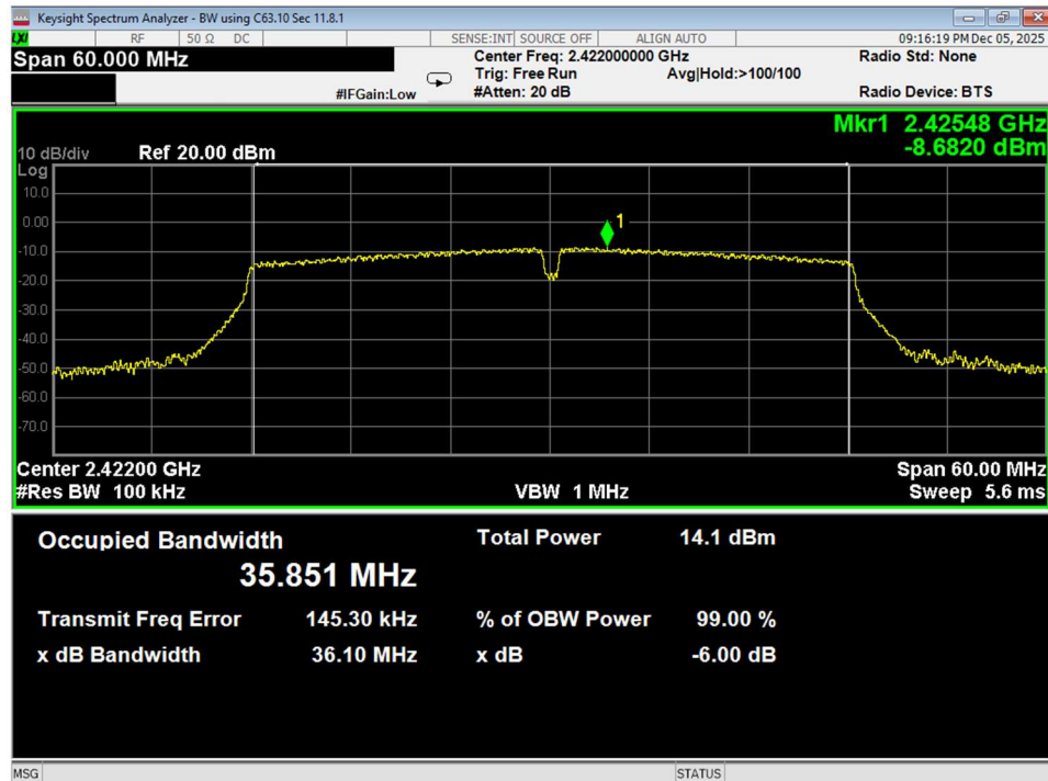
Figure 82 6dB Bandwidth, Low, Wifi N, 40MHz bandwidth, conducted
