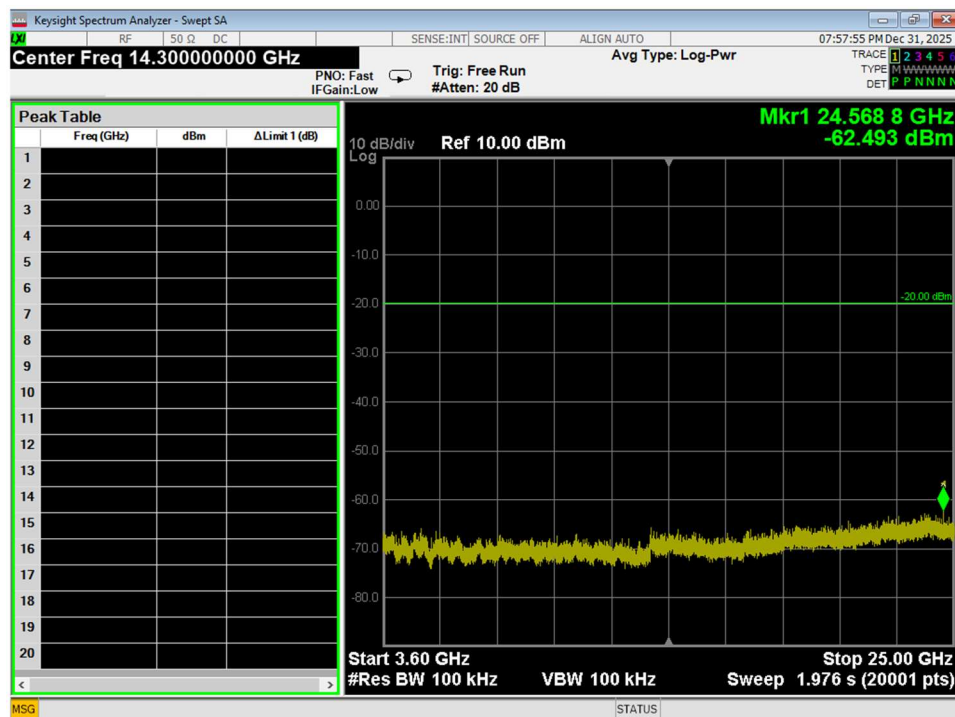
Figure 75 Conducted Spurious Emissions, Wifi N, Mid Channel, conducted, 3.6GHz – 25GHz
