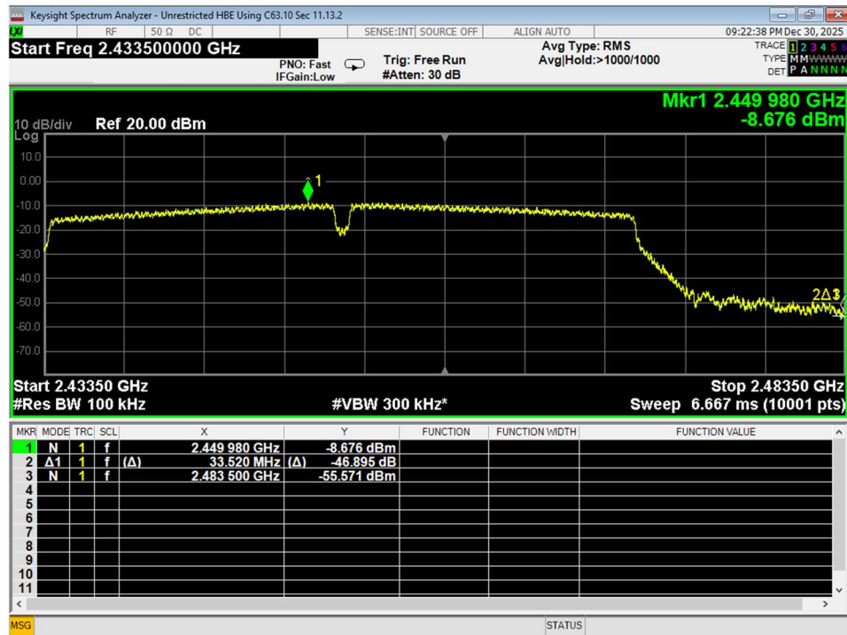
Figure 91 Higher Bandedge, Unrestricted, Wifi N, 40MHz bandwidth, conducted
