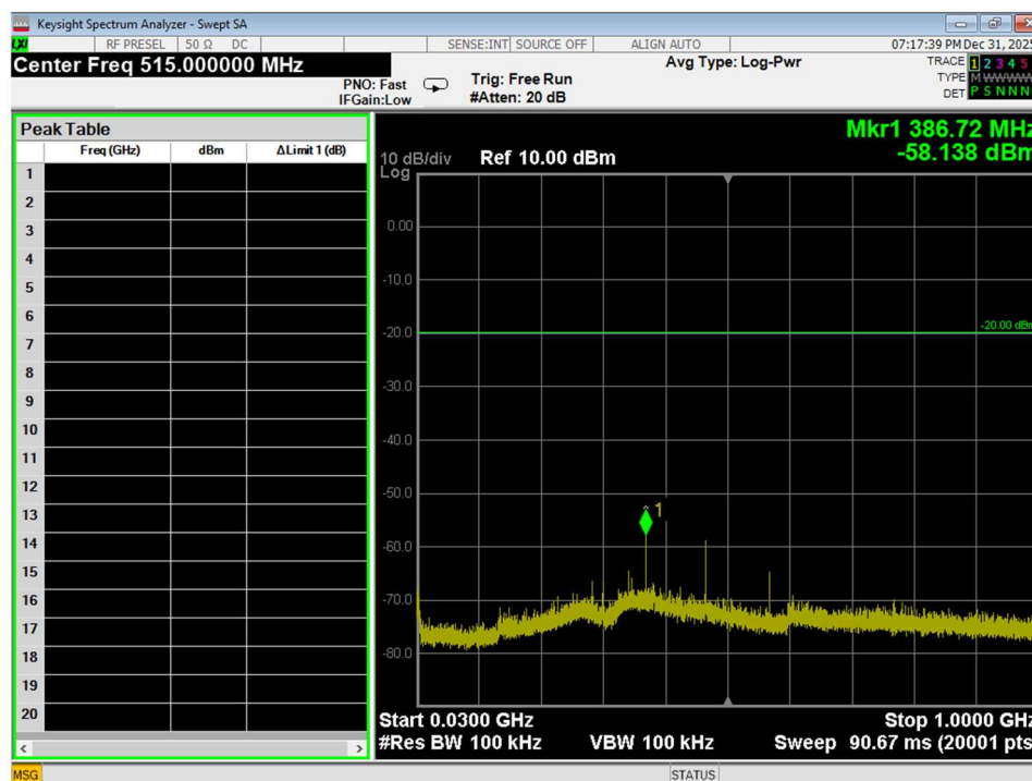
Figure 98 Conducted Spurious Emissions, Wifi N, 40MHz Bandwidth, High Channel, conducted, 30MHz – 1GHz
