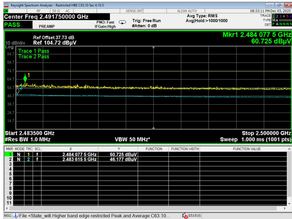
Figure 89 Higher Bandedge, Restricted, WiFi N, 40MHz bandwidth, radiated
