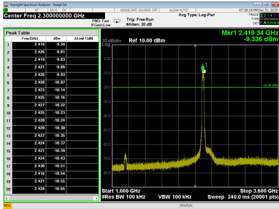
Figure 93 Conducted Spurious Emissions, Wifi N, 40MHz Bandwidth, Low Channel, conducted, 1GHz – 3.6GHz
