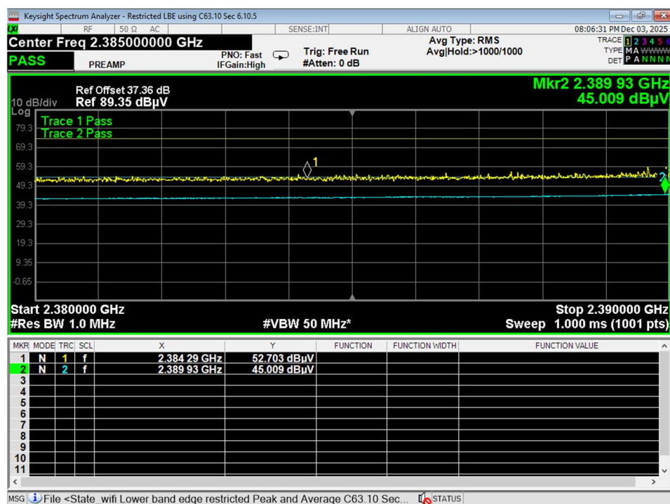
Figure 88 Lower Bandedge, Restricted, Wifi N, 40MHz bandwidth, radiated
