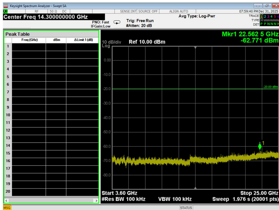
Figure 78 Conducted Spurious Emissions, Wifi N, High Channel, conducted, 3.6GHz – 25GHz
