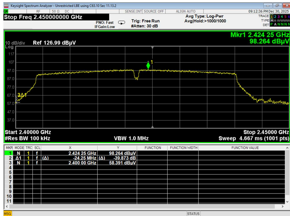
Figure 90 Lower Bandedge, Unrestricted, Wifi N, 40MHz bandwidth, conducted
