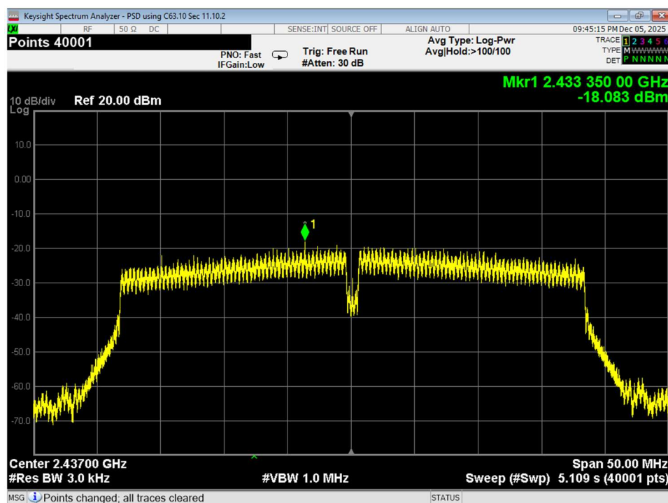
Figure 86 PSD, Mid, Wifi N, 40MHz bandwidth, conducted
