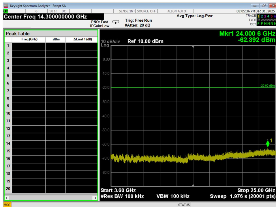
Figure 100 Conducted Spurious Emissions, Wifi N, 40MHz Bandwidth, High Channel, conducted, 3.6GHz – 25GHz
