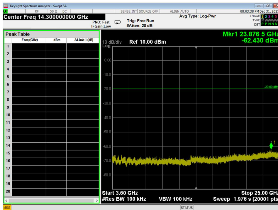
Figure 97 Conducted Spurious Emissions, Wifi N, 40MHz Bandwidth, Mid Channel, conducted, 3.6GHz – 25GHz
