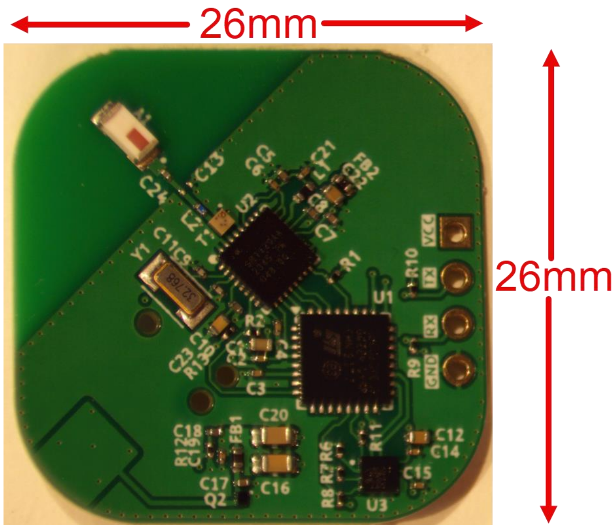
Figure 3. Pet Tag PCBA (Top View)
